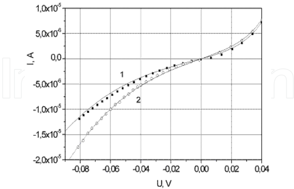
Figure 5. Measured (dots) and calculated (solid lines) current-voltage characteristics of n + -p photodiodes at 77 K. Parameters of traps: E_t=0.72E_g , C_p=1 \cdot 10^{-7} \text{ cm}^3/\text{s} , C_n=0.01C_p , N_t=3.2 \cdot 10^{15} and 4.8 \cdot 10^{15} \text{ cm}^{-3} for curves 1 and 2, respectively.
