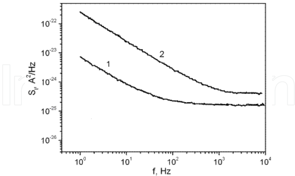
Figure 6. Noise spectra for the photodiodes with R_0A=1.0 \Omega \text{ cm}^2 (1) and R_0A=0.3 \Omega \text{ cm}^2 (2) at 77 K.
