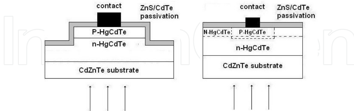
Figure 1. Schematic cross section of mesa (left) and planar (right) HgCdTe IR photodiodes. The photodiodes are illuminated through the wide bandgap substrate.
