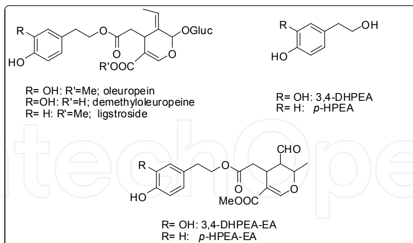
Figure 1. Chemical structures.
