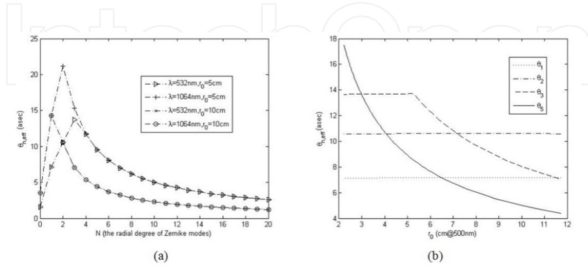
Figure 4. The characteristic angles of the angular anisoplanatism for separated beacon and target. (a) the effective offset angles at different turbulent intensities and wavelengths; (b) the relationship between effective offset angles and turbulence intensities for four different compensational orders at \lambda=532nm
