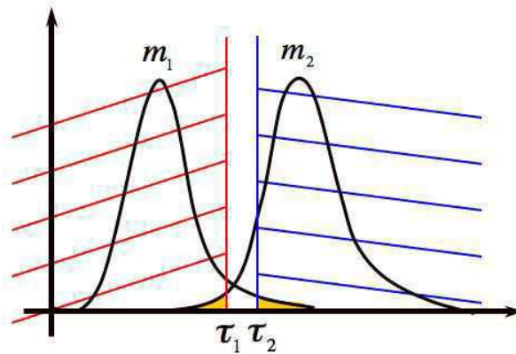
Figure 4. Illustration of the discrimination efficiency criterion. \tau_1 and \tau_2 are defined such that the yellow area under the curve represents 0.05 of the total area under the curves for models m_2 and m_1 , respectively. The discrimination efficiency is defined as the area under the m_i curve delimited by the threshold \tau_i , as a percentage of the total area under the model m_i curve.
