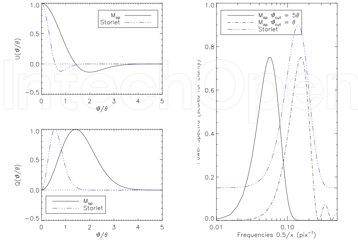
(a) M_{ap} and wavelet filter functions in real space
