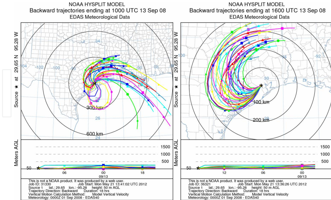
Figure 14. Back trajectory ensembles for 04:00 CST (left) and 10:00 CST (right) on DOY 257.
