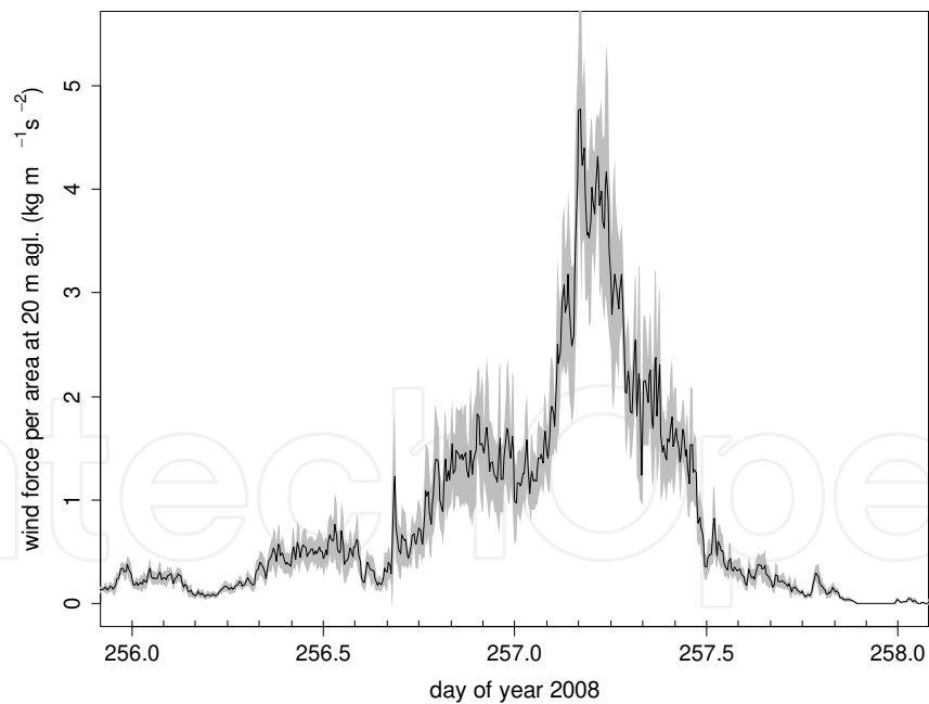
Figure 6. Wind force, proportional to \hat{U}^2 , time series during Hurricane Ike's passage over Houston. The grey swath is an estimate of its standard deviation.
