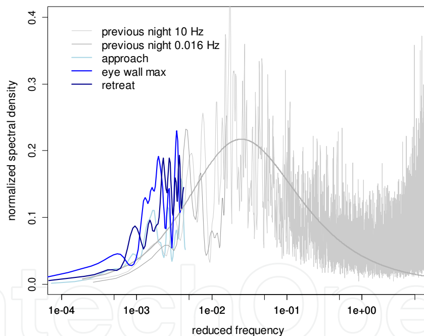
Figure 8. A comparison of longitudinal wind speed spectra between the night before the hurricane (DOY 256, hours 01:00-03:00 CST) and three periods of the highest encountered wind speeds before, during, and after the eyewall maximum. Smoothing was limited to highlight differences. The thick, dark grey line represents a standard spectrum. Note that the grey spectra from the previous night were obtained at an average wind speed of 6 \text{ m s}^{-1} , the offset being due to a slightly higher value recorded by the cup anemometer. Wind speeds for the blue spectra were all above 22 \text{ m s}^{-1} (Fig. 3). To match power density levels (y-axis) the blue spectra were additionally normalized to the wind speeds' standard deviation ratios.
