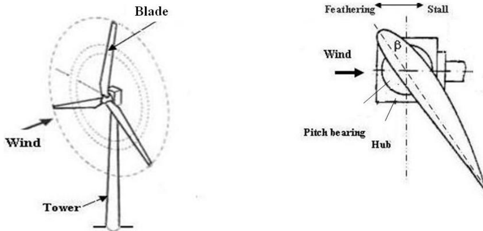
Figure 1. Limiting power output using pitch control.
