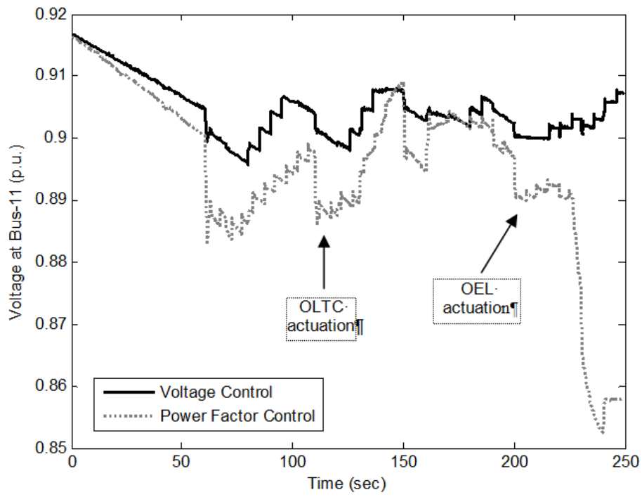
Figure 13. Voltage at Bus 11.
