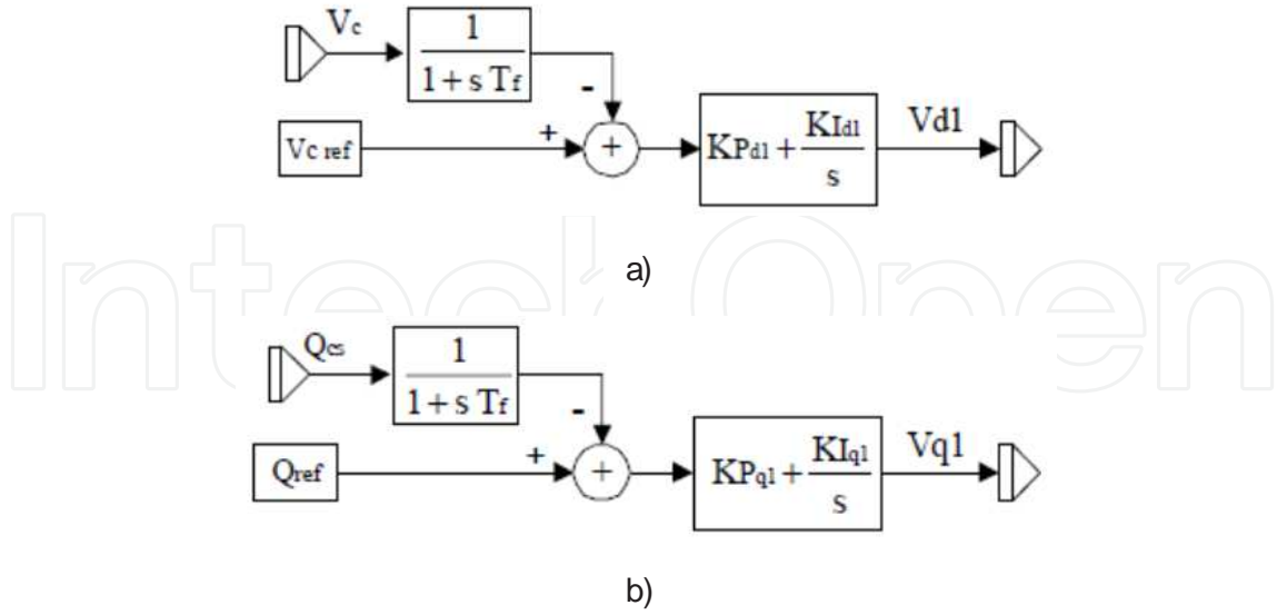
Figure 2. Control loop of the stator side converter (SSC) a) Component V_{d1} b) Component V_{q1} .
