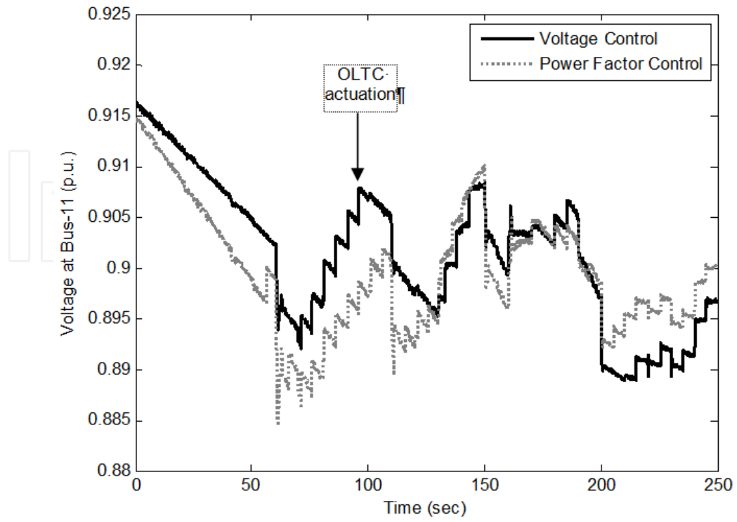
Figure 7. Voltage at bus 11
