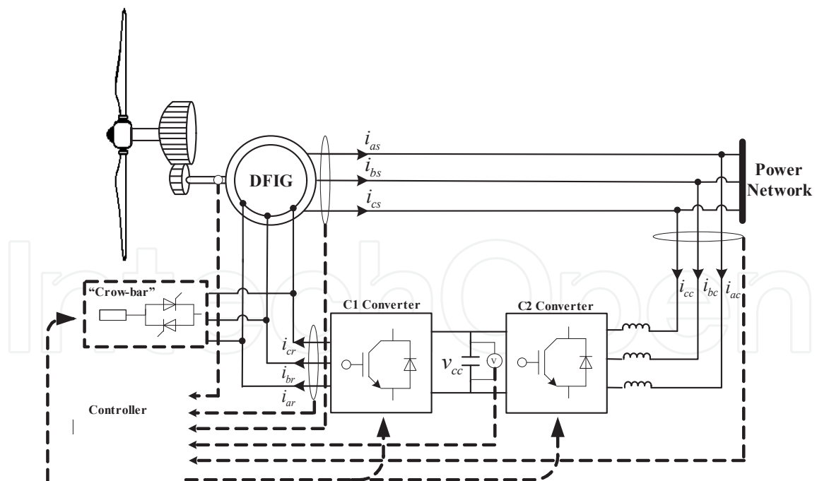
Figure 1. DFIGs Scheme
