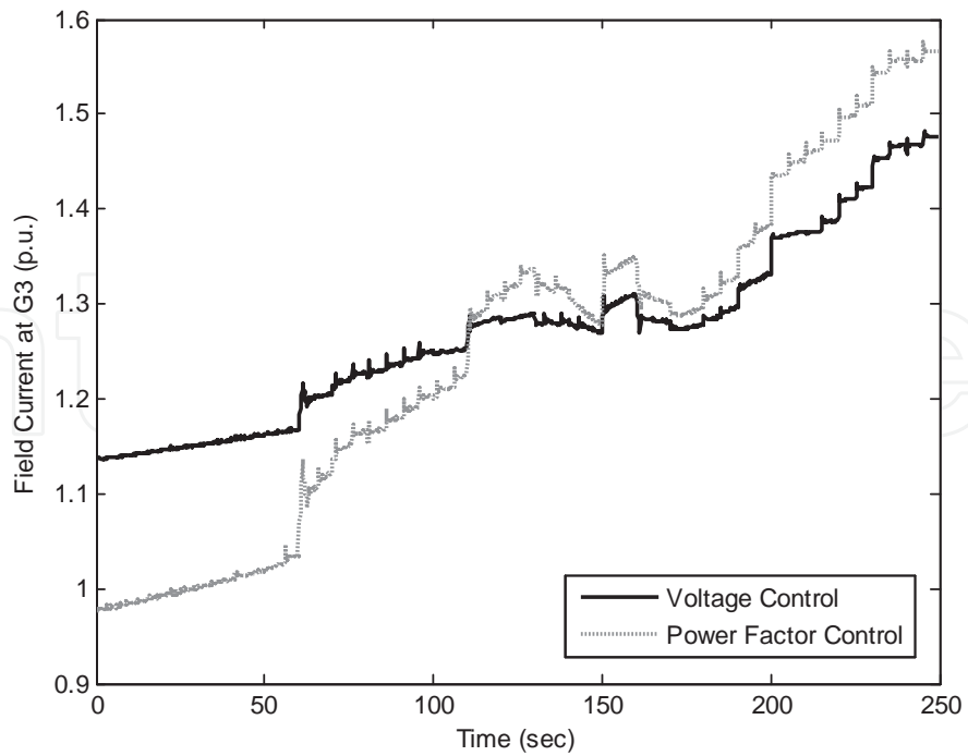
Figure 10. Field current at G3.
