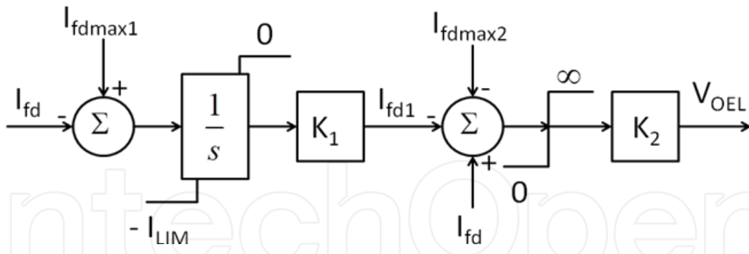
Figure 4. OEL model.
