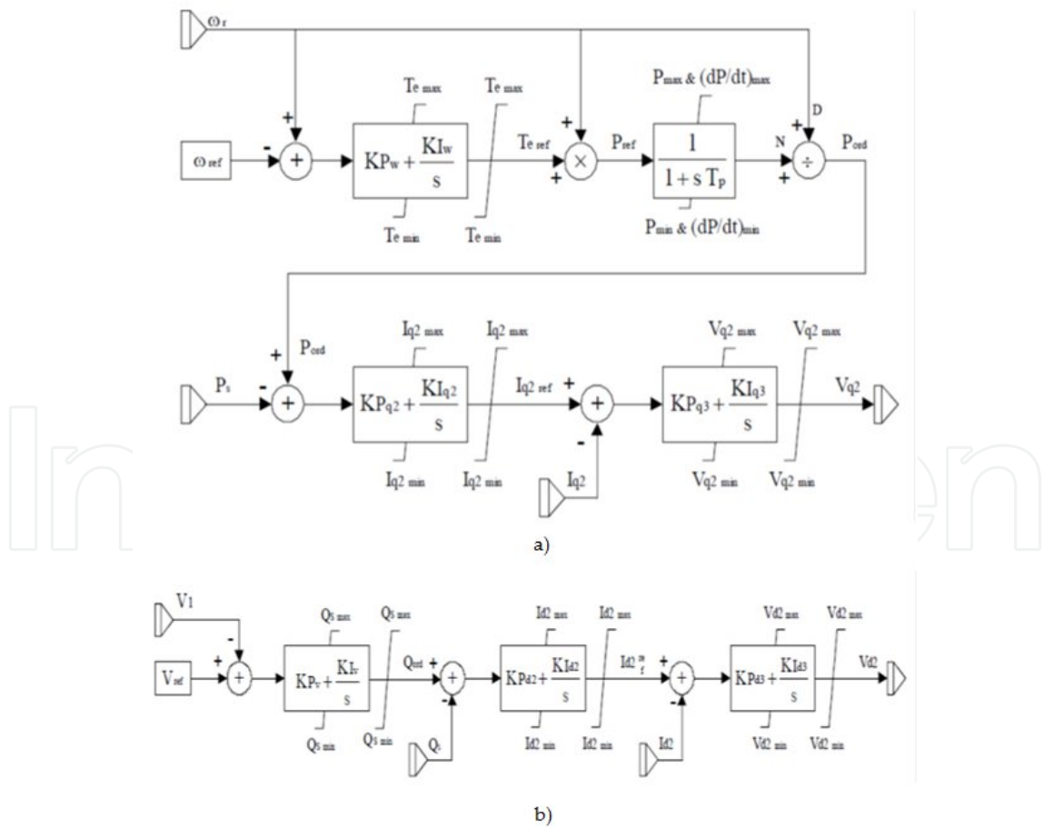
Figure 3. Control loop of the rotor side converter (RSC) a) Component I_{q2} b) Component I_{d2} .
