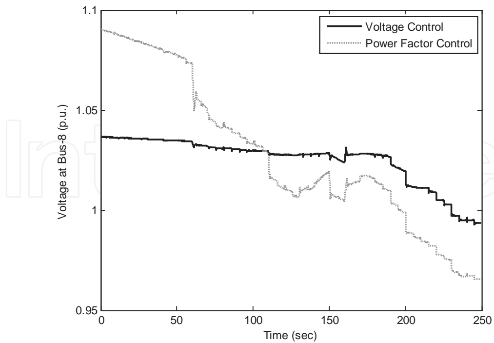
Figure 8. Voltage at bus 8
