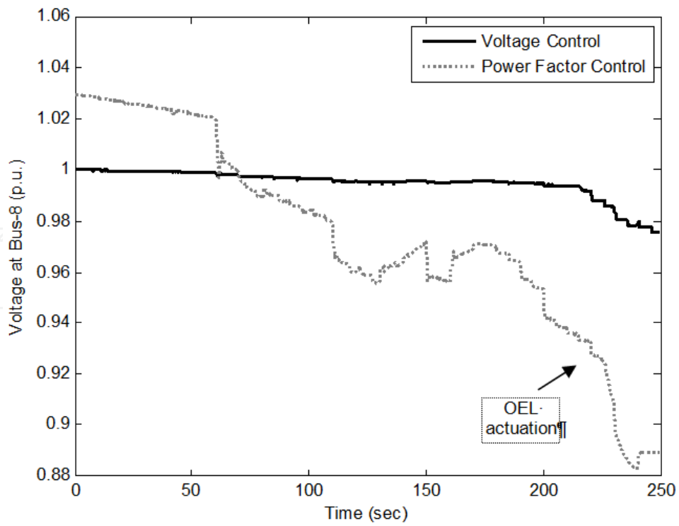
Figure 14. Voltage at Bus 8.
