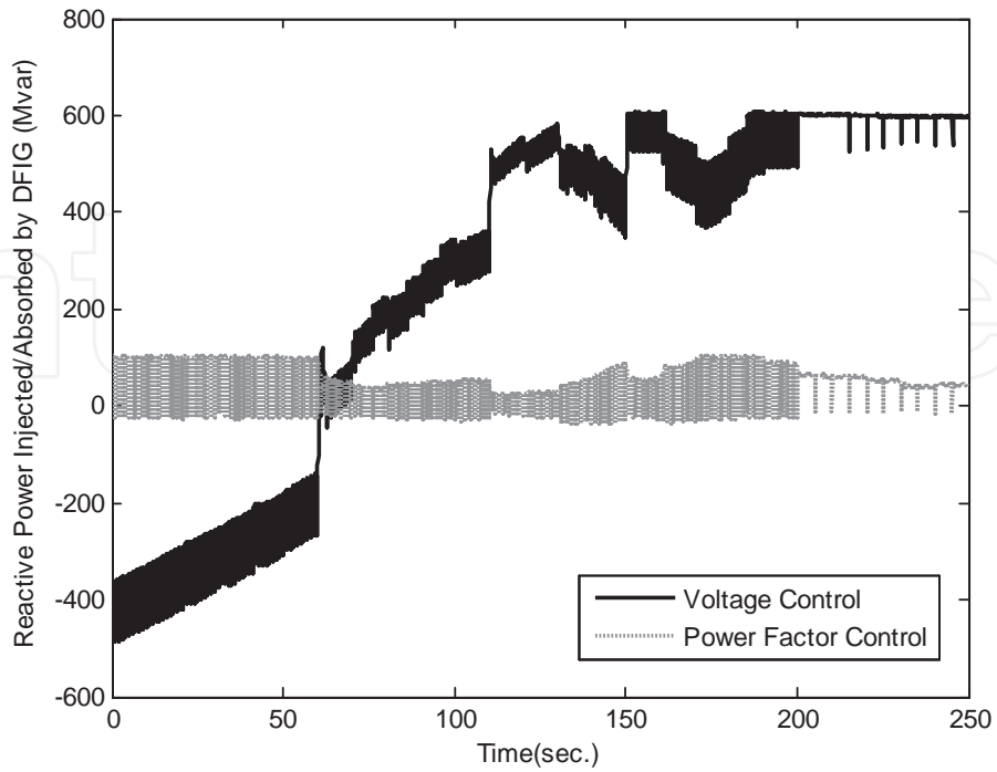
Figure 9. Reactive power injected / absorbed by DFIG.
