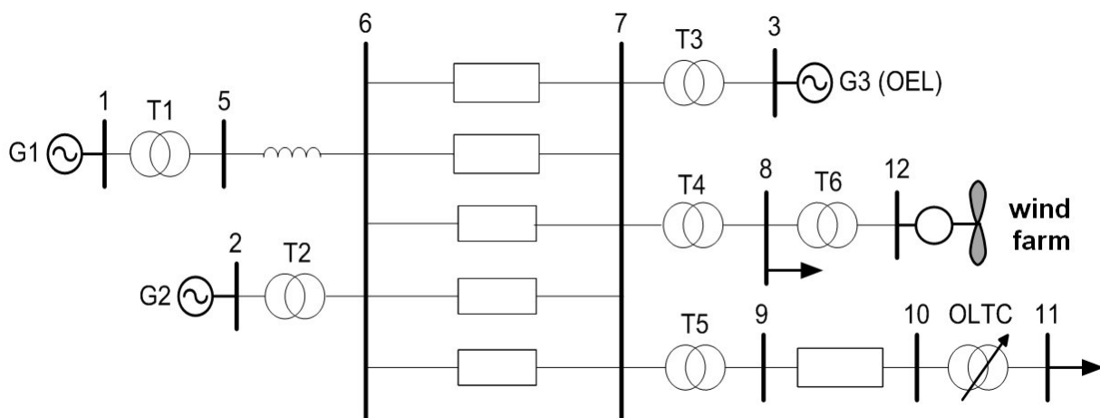
Figure 5. Test system diagram.
