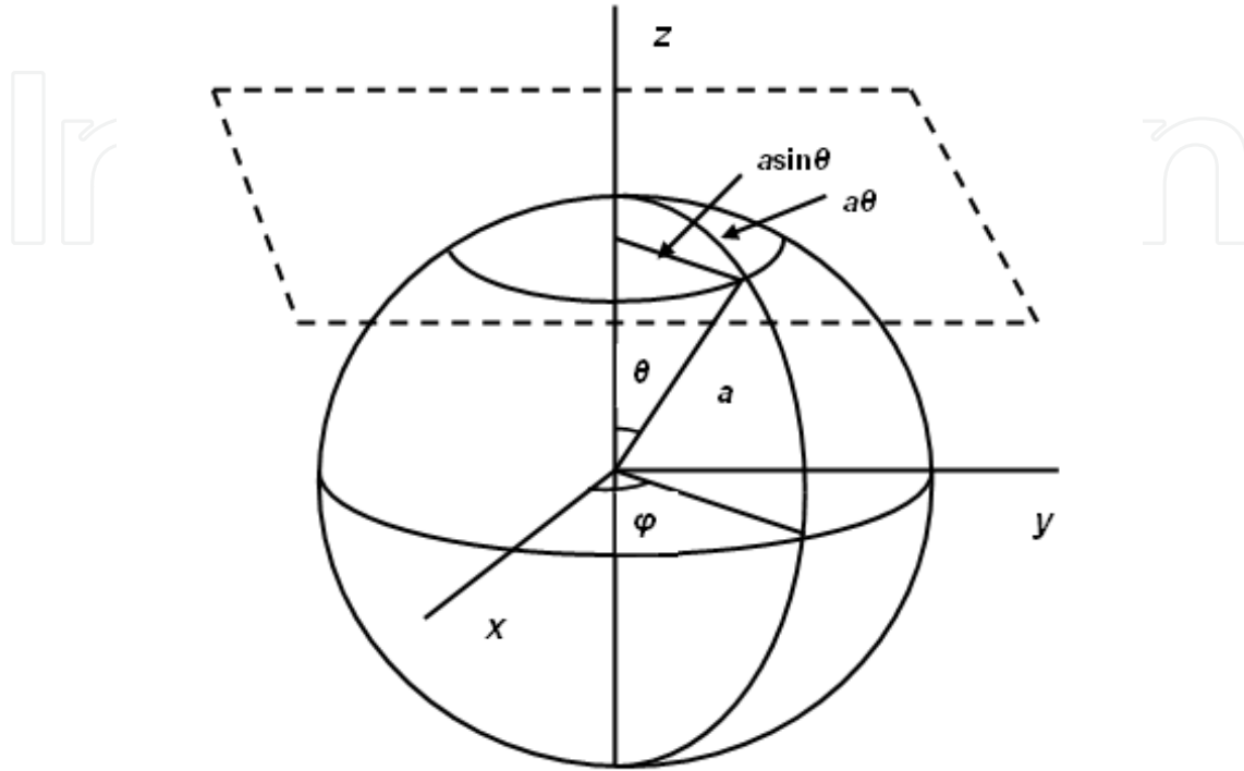
Figure C.1. Spherical surface with source at north pole ( \theta = 0 ).
