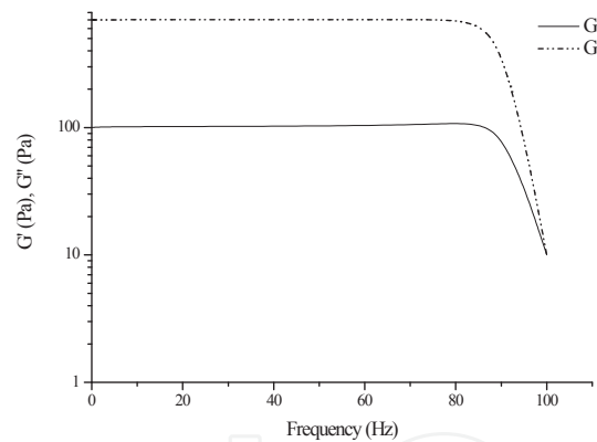
Figure 15. A frequency sweep example ( G'' > G' ).
