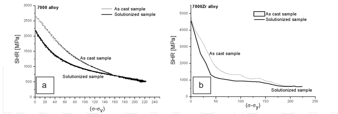
Figure 7. Strain hardening rate curves for the RT tensile curves of 7000 (a) and 7000Zr (b) alloy in the as-cast and solutionized state.
