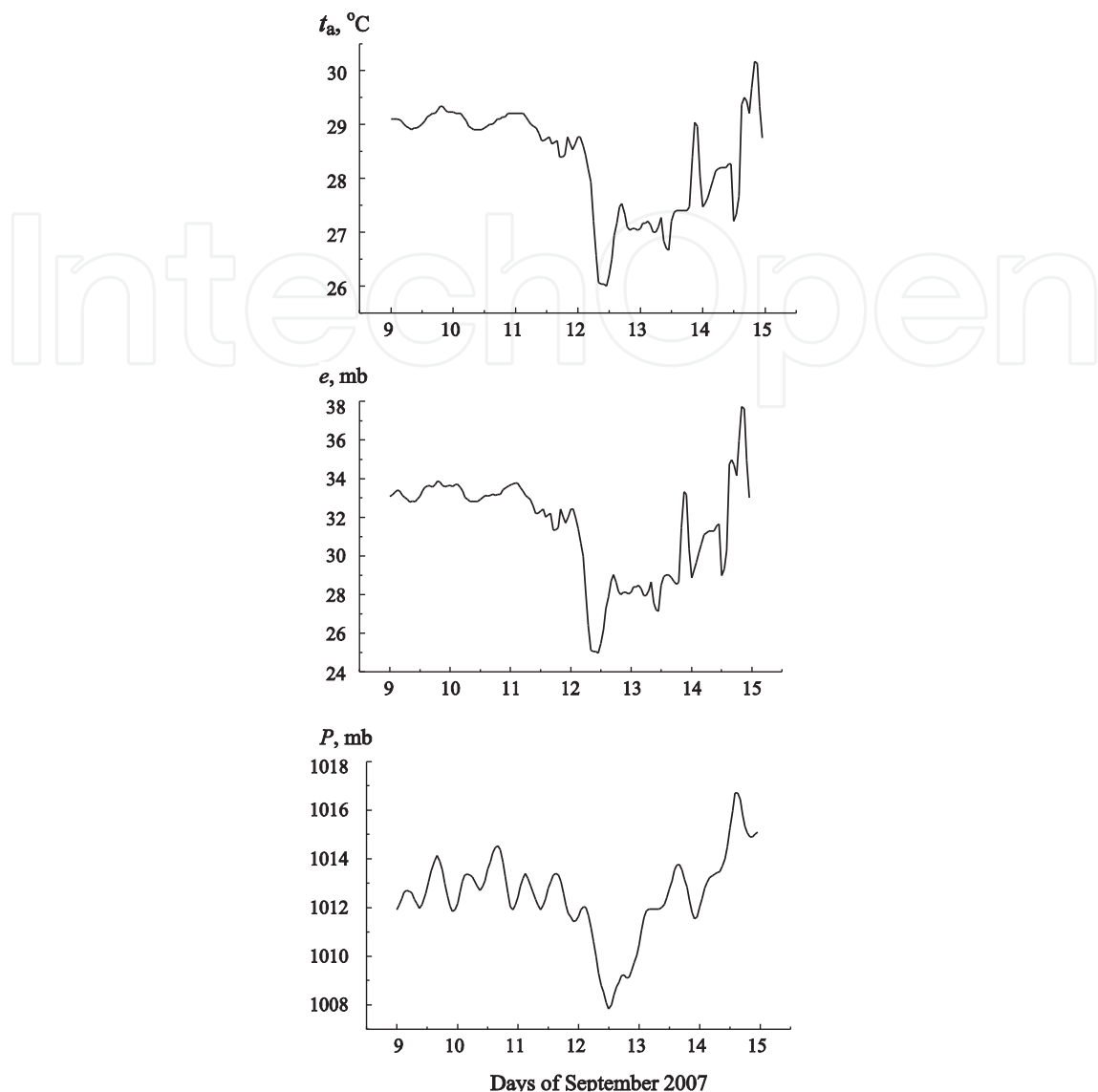
Figure 2. Variations of the near-surface temperature t_a , humidity e , pressure P from the measurement data of the station 42019 in the Gulf of Mexico during the starting the TH Humberto in September 2007.
