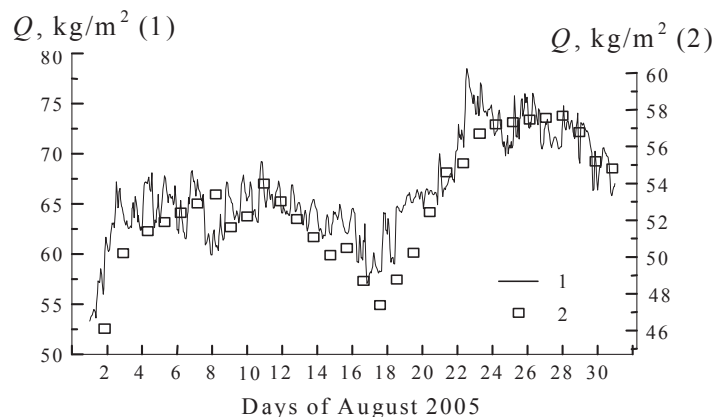
Figure 7. Comparing the estimates of the atmosphere integral water vapor content Q in area of the station SMK1: 1 - data of computing for the layer 10:10000 m; 2 - data of measurements of the radiometer SSM/I.
