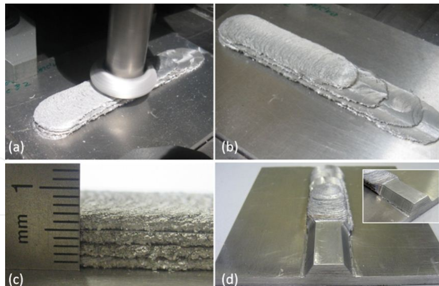
Figure 8. Build-up by friction surfacing. a) Successive deposition; b) Bulk produced from four overlapped passes; c) Detail of final thickness achieved; d) Milling of linear rail.
