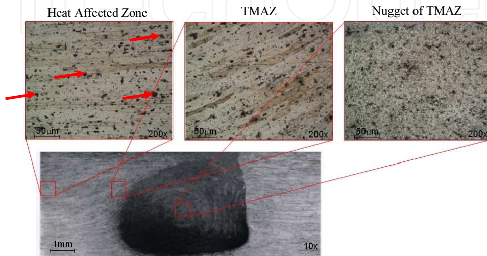
Figure 13. Metallurgical analysis of a FSW of AA2024-T3 (thickness = 4.8 mm), \Omega = 1120 rpm, v = 320 mm/min. The arrows in the HAZ detail are identifying some of the several precipitates.
