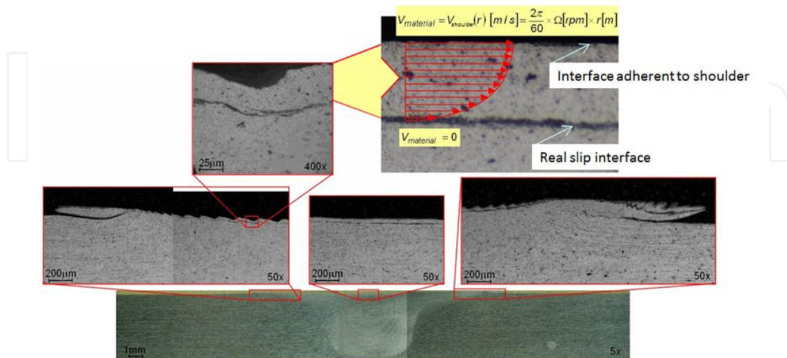
Figure 16. Superficial layer of weld bead material in contact with shoulder that is dragged to rotate along with the shoulder generating a real slip interface about 10 μm within the material.
