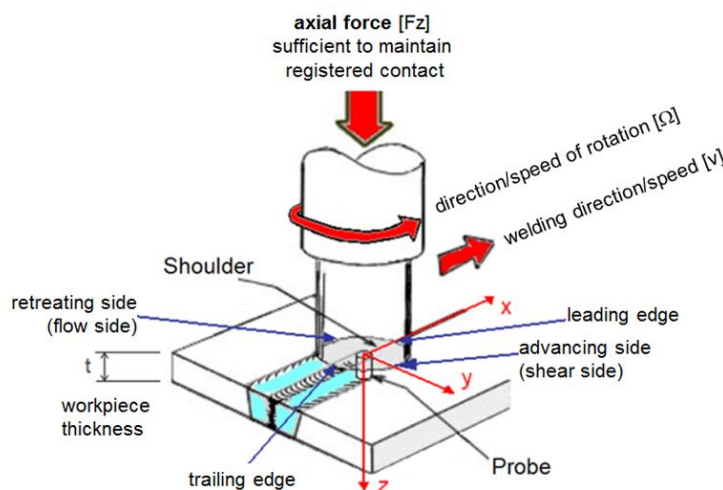
Figure 12. Representation of the main parameters and nomenclature of FSW joints.
