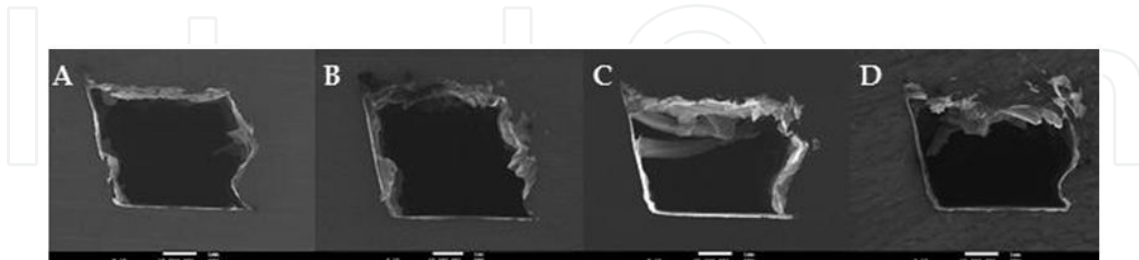
Figure 26. Cross section macrograph showing the channel geometry at different FSC processing parameters for the same FSC tool: a) 600 rpm, 80 mm/min.; b) 600 rpm, 150 mm/min.; c) 800 rpm, 80 mm/min. and d) 800 rpm, 150 mm/min.
