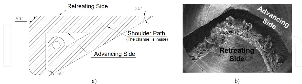
Figure 31. Slope paths. a) linear sloped path tested and b) result of the visual inspection after milling a hole at the 90 degree corner.
