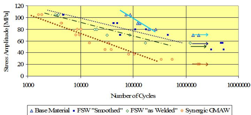
Figure 19. S-N curves from fatigue test trials ( R=0.1 ; f=20\text{Hz} ) of different testing conditions of AA5083-H111 (thickness = 4 mm).
