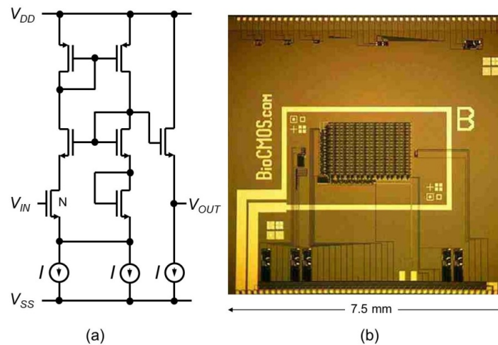
Figure 2. (a) Basic CMOS source-drain follower. V_{DD} and V_{SS} are high and low power supply voltages, respectively. (b) 16 \times 16 integrated sensor array with CMOS source-drain followers and peripheral circuits. A heater and thermometer are also integrated on the chip.
