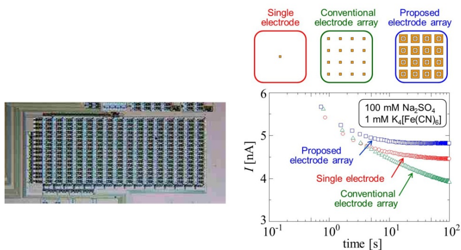
Figure 11. Amperometric sensor array (16×16) and current responses of fabricated microelectrodes. The size of the working electrode is 25×25 μm 2 .
