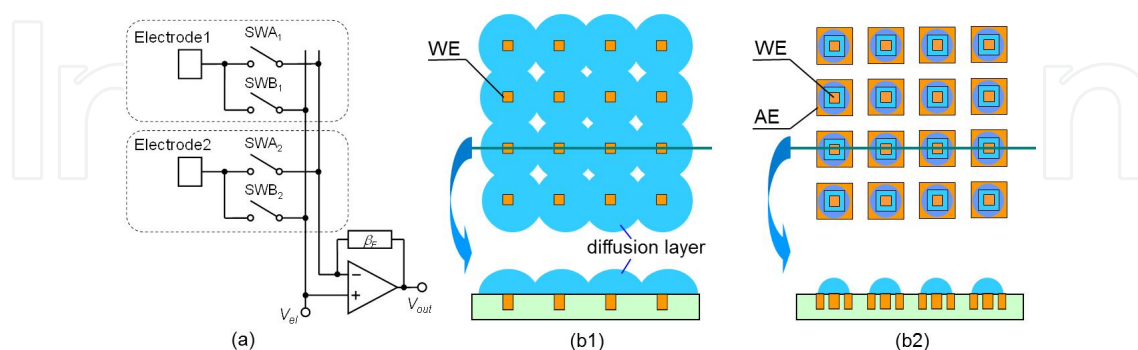
Figure 10. a) Amperometric electrochemical sensor circuit. Each electrode is connected to two switches. (b) Conventional and proposed electrode geometry.
