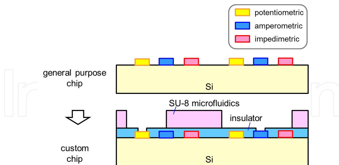
Figure 16. General-purpose sensor chip integrated with potentiometric, amperometric, and impedimetric sensor units. The chip can be customized by the post-CMOS process.
