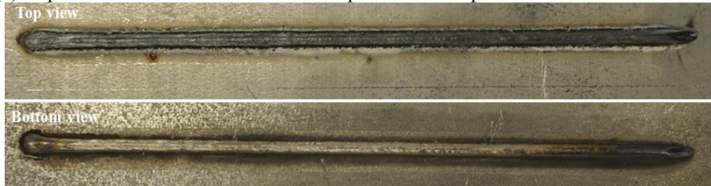
(b) Top and bottom views of the weld acquired under a pressure wheel force of 6 N
