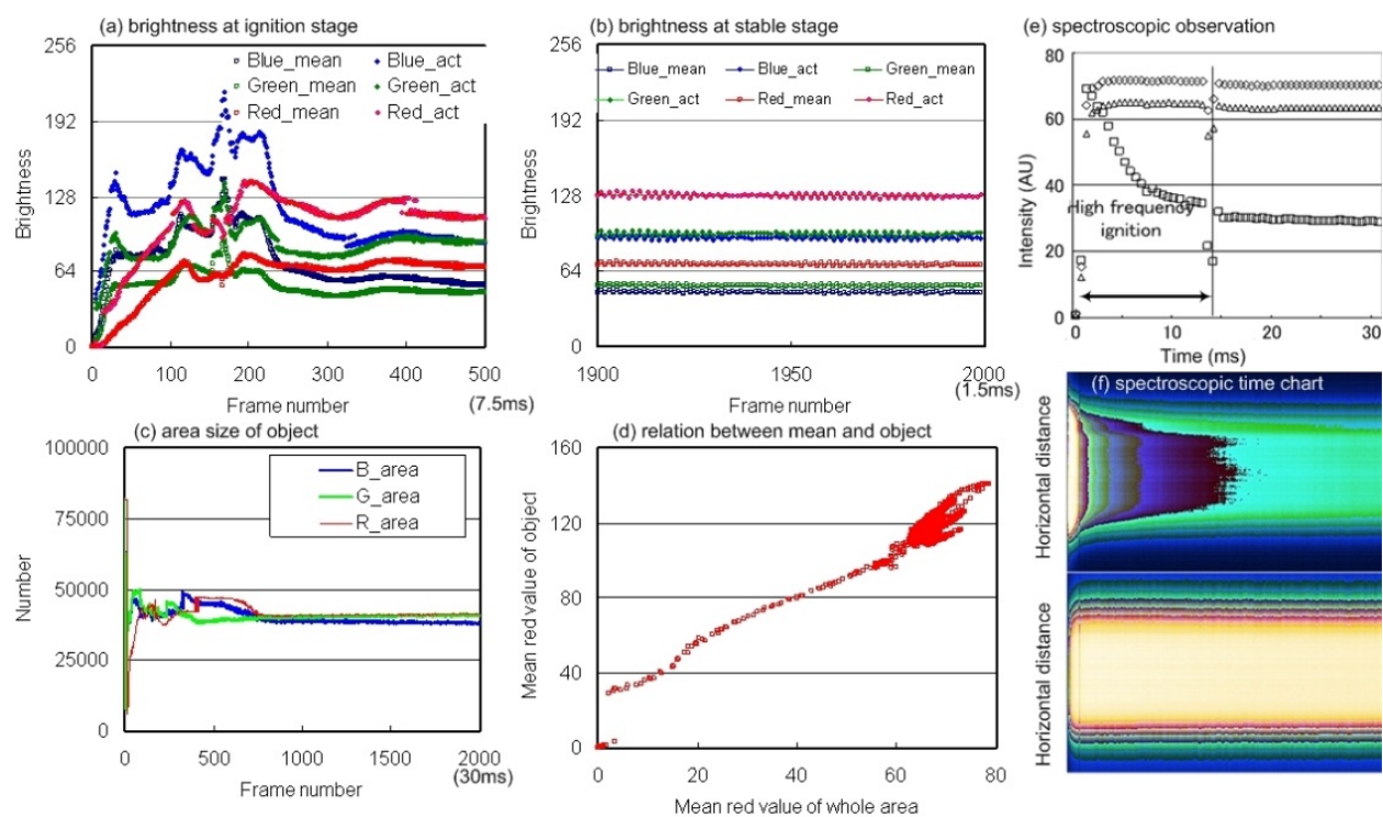
Figure 17. Examples of brightness characteristics.
