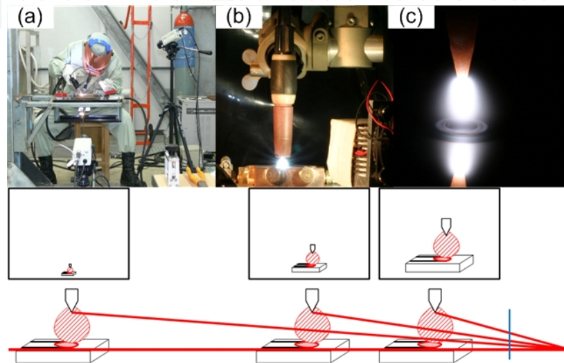
Figure 2. Size effect on image quality.
