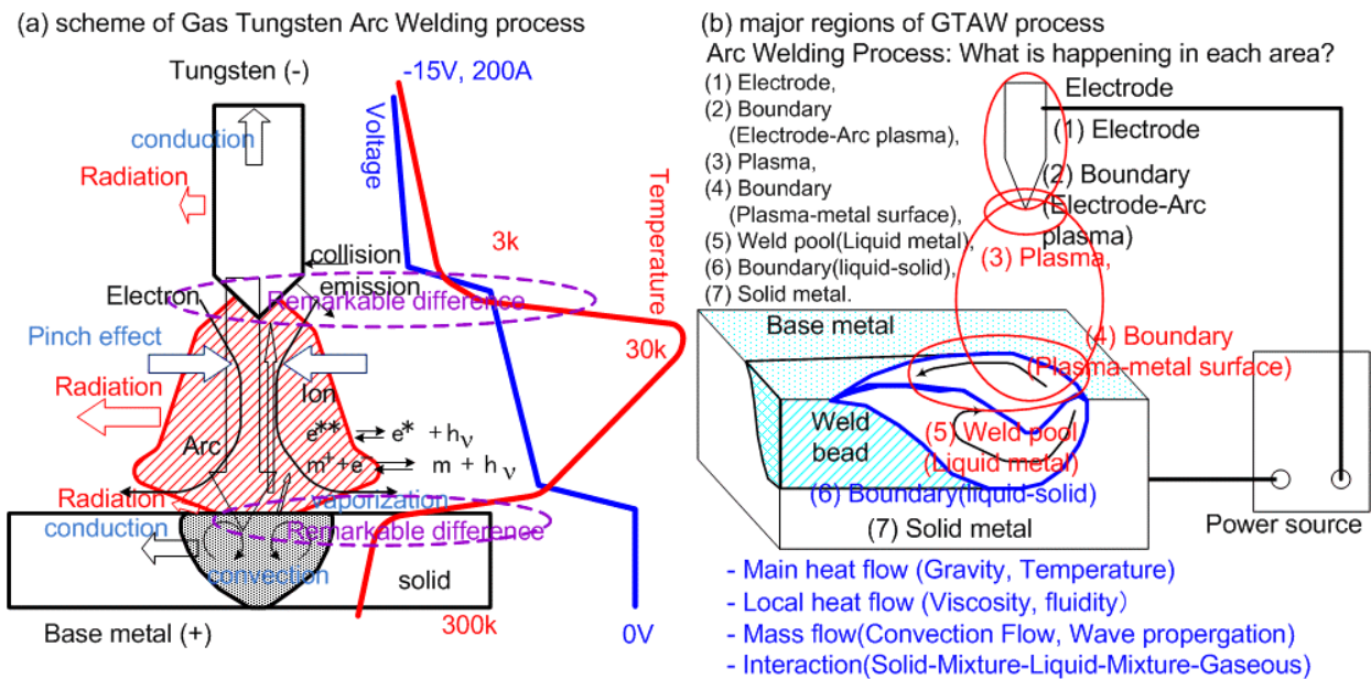
Figure 1. Scheme of Gas Tungsten Arc Welding(GTAW) process.
