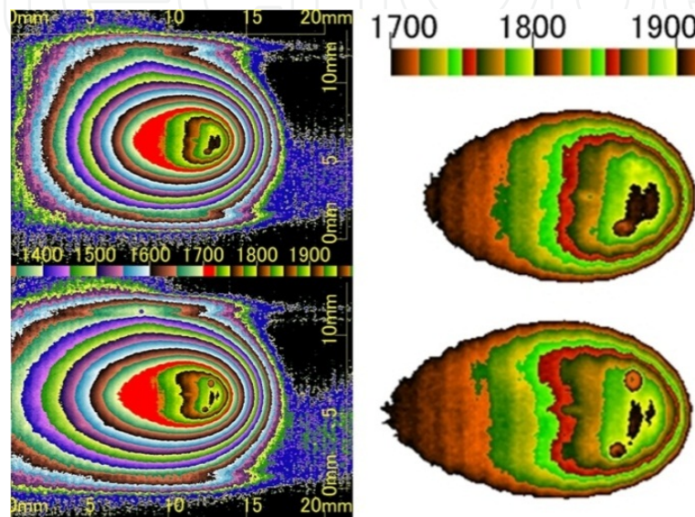
Figure 24. Pseudo colour image of temperature distribution.
