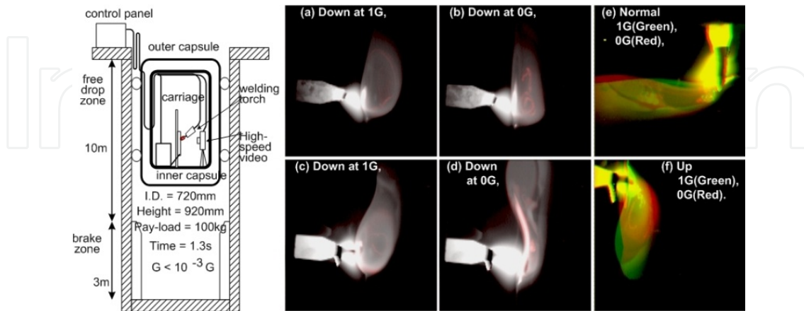
Figure 29. Results of drop tower experiment.
