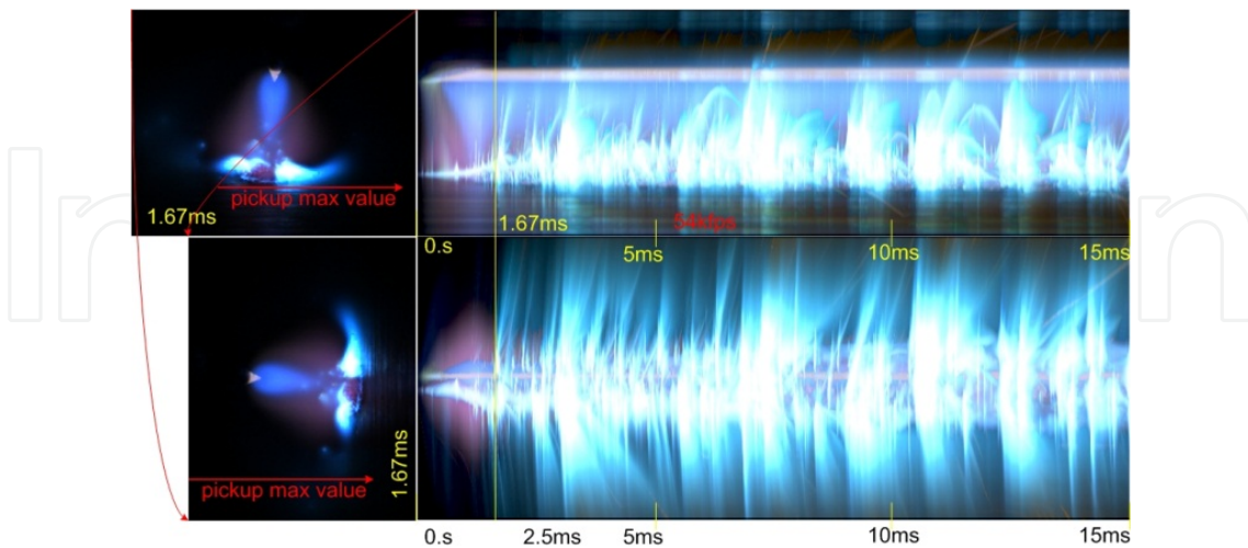
Figure 11. Example of time charts to recognize arc ignition stage in air.
