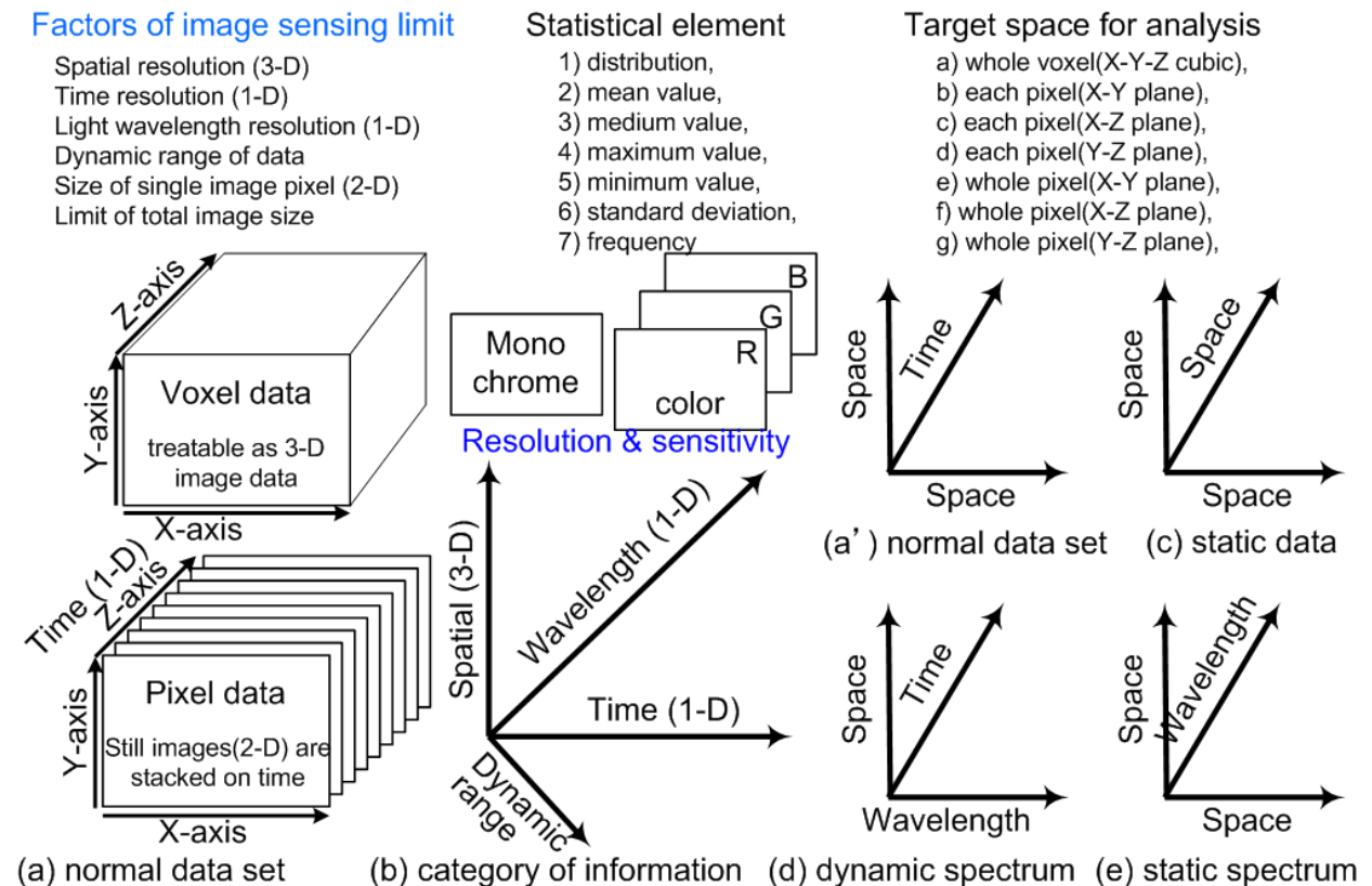
Figure 3. Data structures of high speed imaging.
