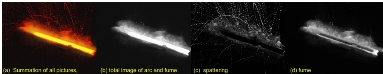
Figure 32. Example of imaging methods..
