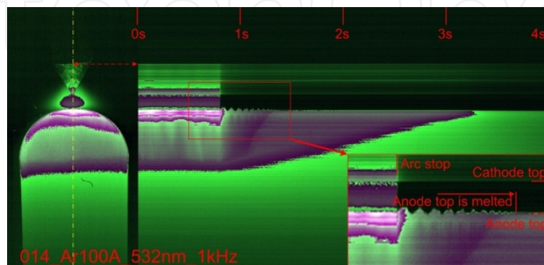
Figure 20. Dynamic response of thermal radiation.
