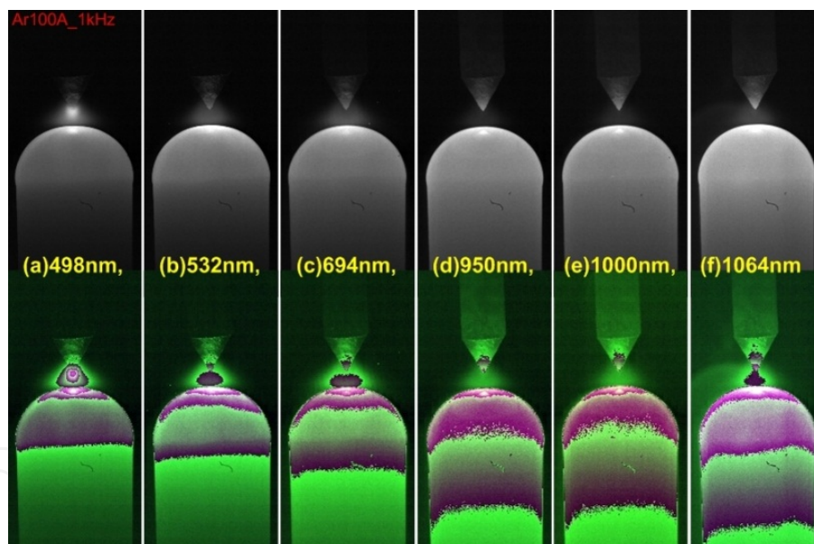
Figure 21. Effect of wavelength on radiation.
