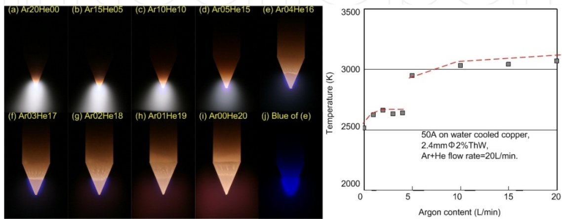
Figure 18. Effect of gas contents on arc behaviour.
