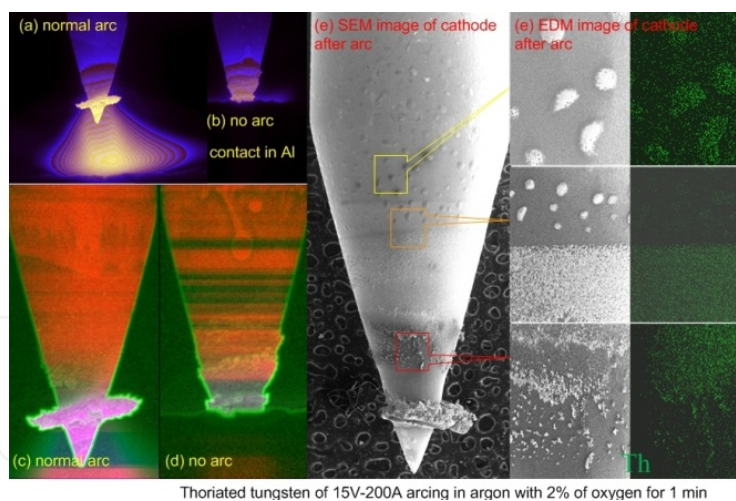
Figure 28. Effect of oxygen for reactions on cathode.
