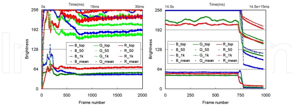
Figure 16. Time response of brightness in each frames.
