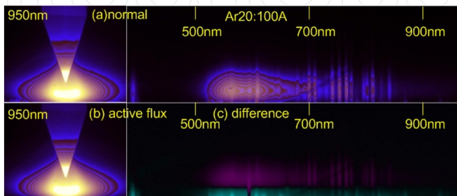
Figure 27. Effect of active flux on arc plasma.
