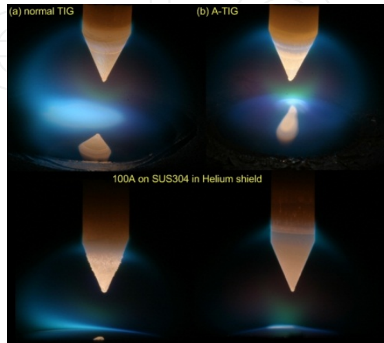
Figure 25. Effect of active flux on arc process.
