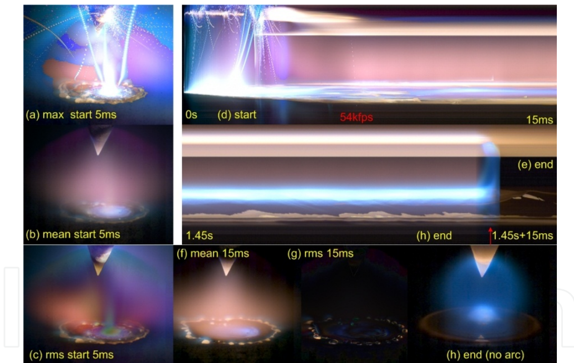
Figure 12. Methods to show process behaviour GTAW in helium shield.
