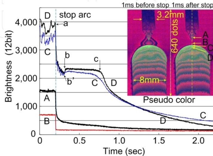
Figure 22. Measurement of surface temperature.
