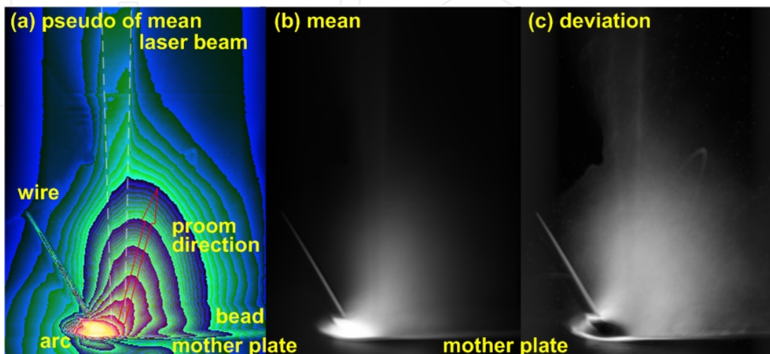
Figure 33. Statistical image of laser arc hybrid welding.
