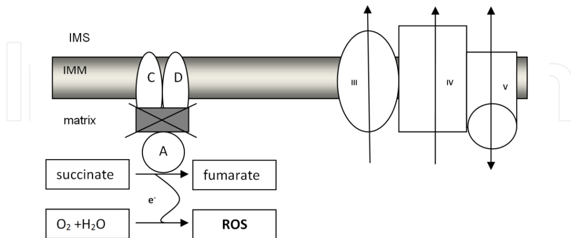
Figure 11. ROS model [18].
