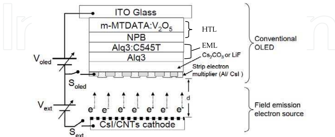
Figure 10. Schematic presentation of an apparatus for characterizing a FEOLED with strip electron multiplier
