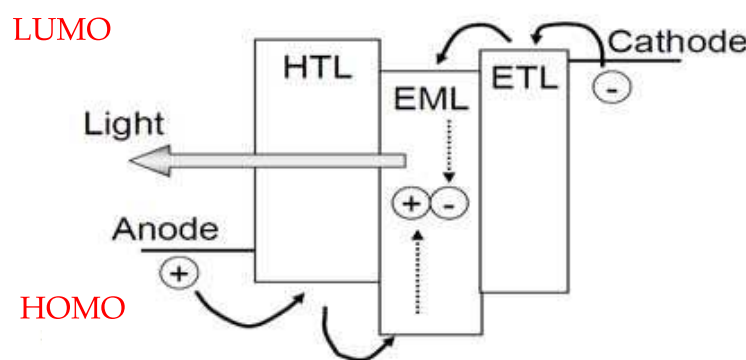
Figure 3. Schematic sketch of the active energy levels of organic light emitting diodes (OLEDs)
