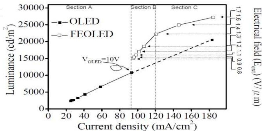
Figure 13. The Luminance (L)-Current density (J)-Electric field (E) of the OLED and FEOLED devices at both S_{oled} and S_{ext} close ( E_{ext}=V_{ext}/d ) (Fig. 10)
