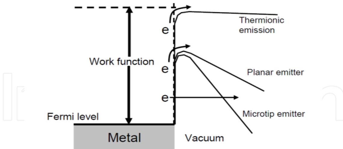
Figure 1. Schematic diagram of the field emission barriers for a planar and a micro-tip emitter.
