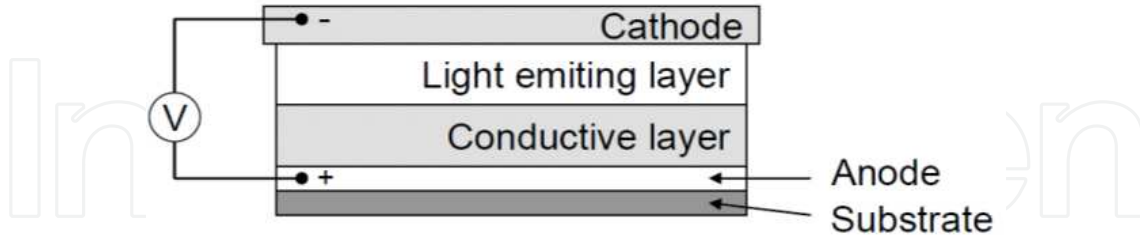
Figure 2. Schematic structure of organic light emitting diodes.
