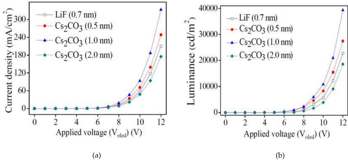
Figure 11. (a) Current density (J)-Applied voltage (V) at SOLED closes and Sext is open and (b) Luminance (L)-Applied voltage (V) at Soled=closes and Sext is open(Fig.10)
