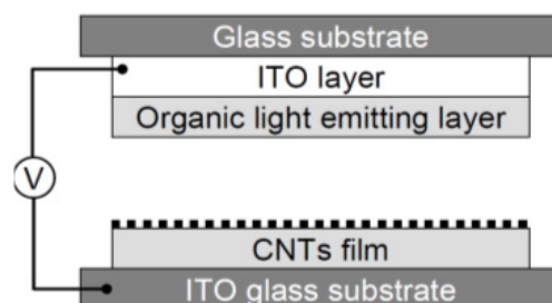
Figure 4. The schematic diagram of a FEOLED.
