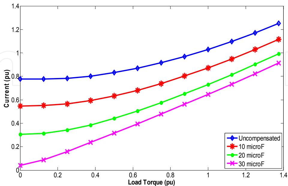
Figure 8. Torque–Current waveform
