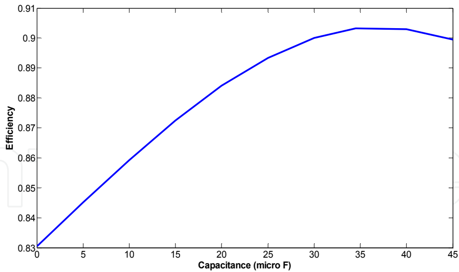
Figure 11. Capacitance-Efficiency waveform
