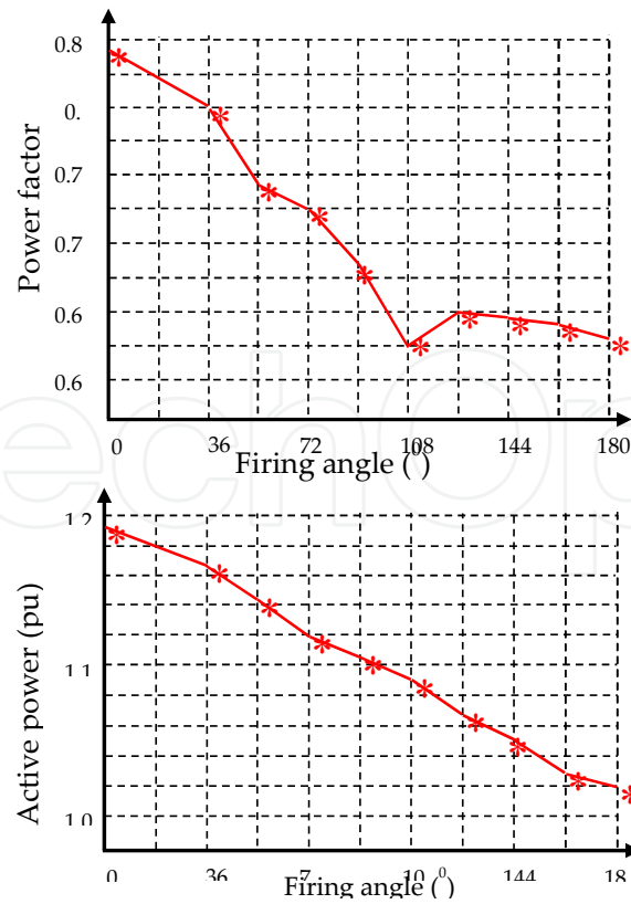
Figure 20. Experimental results of power factor and active power versus firing angle
