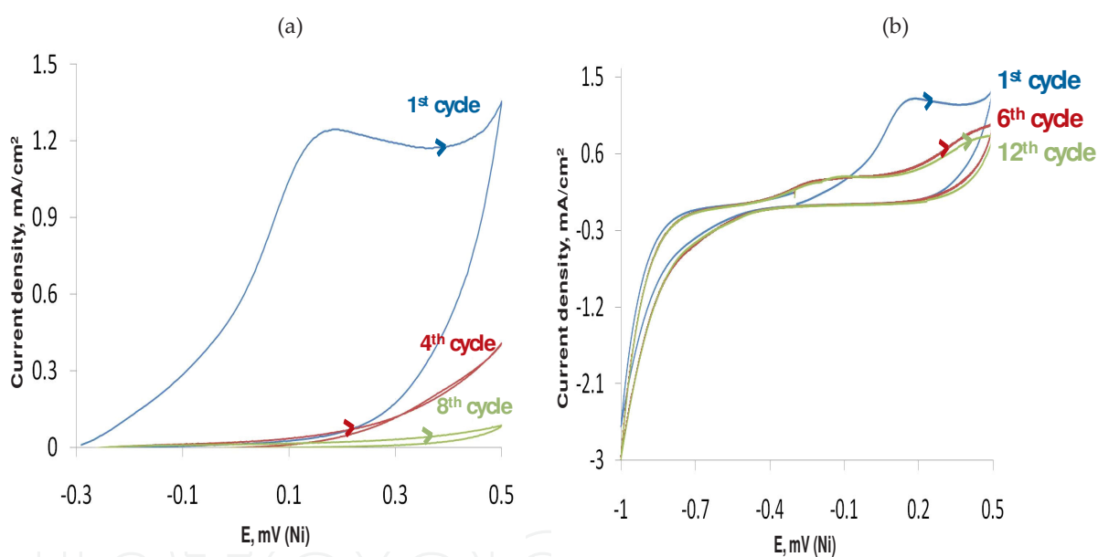
Figure 7. Successive cyclic voltammograms of Ni electrode in CBS (pH 6.4) in presence of 120\text{ mM} \text{NaCl} . Scan rate: 100\text{ mV/s} . (a) potential range: -0.3\text{ V} \rightarrow 0.5\text{ V} \rightarrow -0.3\text{ V} and (b) potential range: -0.3\text{ V} \rightarrow 0.5\text{ V} \rightarrow -1.0\text{ V} [adapted from 21].
