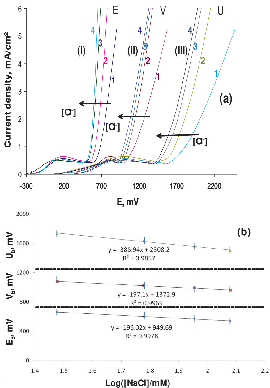
Figure 6. a) (I) j vs. E , (II) j vs. V , and (III) j vs. U ( = E+V ), where j is the current density, after sweeping the potential between -0.3\text{ V} \rightarrow 0.8\text{ V} vs. SCE in CBS (36 mM, pH 7) and in presence of NaCl (curves 1: 30 mM, curves 2: 60 mM, curves 3: 90 mM, and curves 4: 120 mM). (b) Evolution of E_b , V_b and U_b as a function of \text{Log}[\text{Cl}^-] (data from Figure 6a) [adapted from 19].
