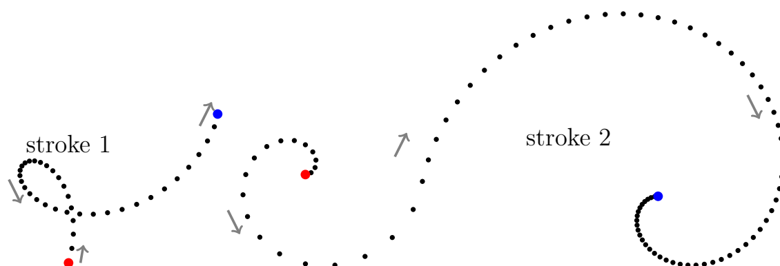
Figure 1. On-line stroke sequences in the form of 2D (x, y) coordinates. In this illustration, initial pen-tip position is coloured with red and pen-up (final point) is coloured with blue.
