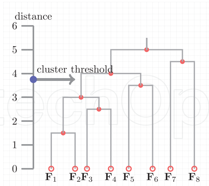
Figure 10. Hierarchical stroke clustering concept. At every step, features are merged according to their similarity up to the provided threshold level.
