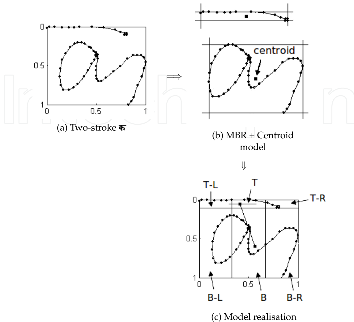
Figure 7. Pairwise spatial relation for a two-stroke क [40].
