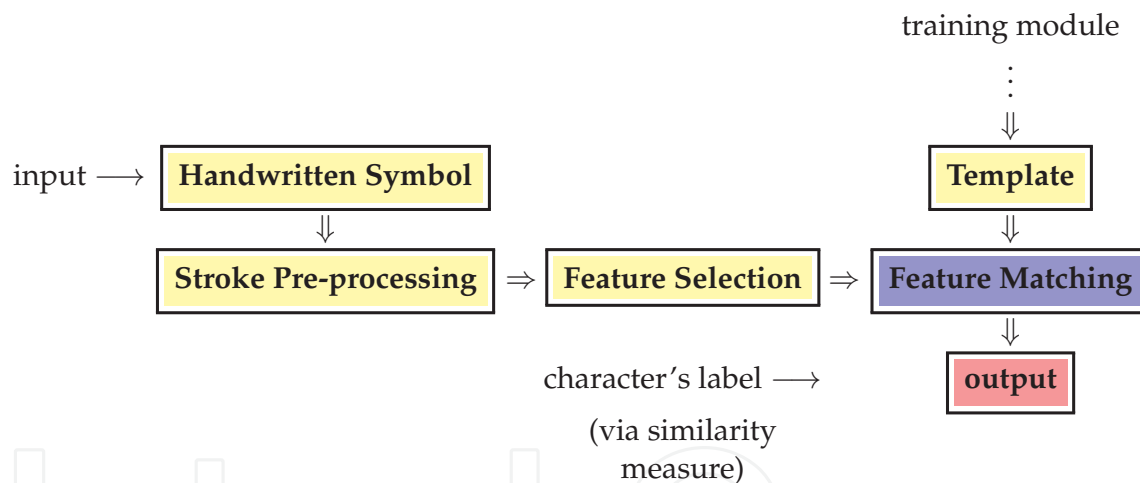
Figure 4. An illustration of testing module. As in learning module, test characters are pre-processed and we present a basic concept to form template via clustering of features of the strokes immediately after they are pre-processed.
