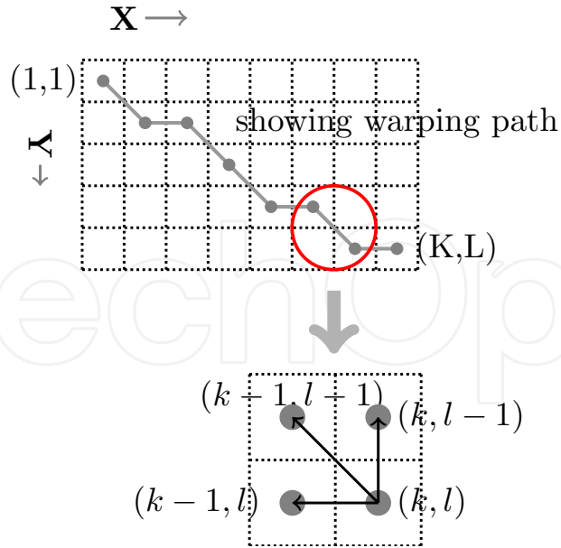
Figure 6. Classical DTW algorithm – an alignment illustration between two non-linear sequences \mathbf{X} and \mathbf{Y} . In this illustration, diagonal DTW-matrix is shown including how back-tracking has been employed.
