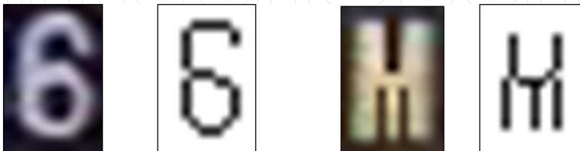
Figure 4. Thinning results using the Zhang-Suen Thinning Algorithm.
