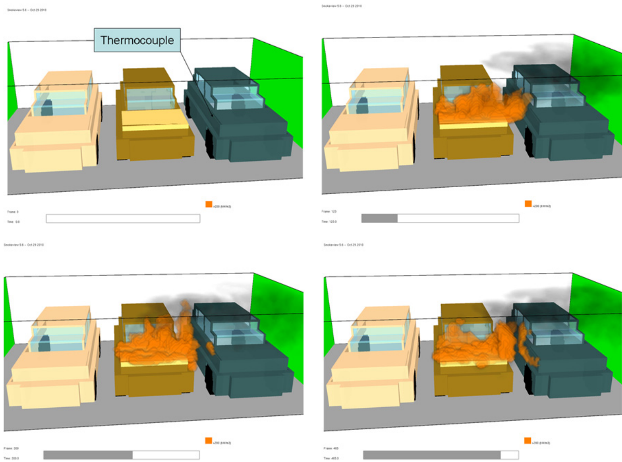
Figure 19. Simulation of near-standing automobile ignition: the case of 45 cm distance between automobiles and 2 m.s -1 air flow velocity in the 0 th , 120 th , 300 th and 465 th s of fire
