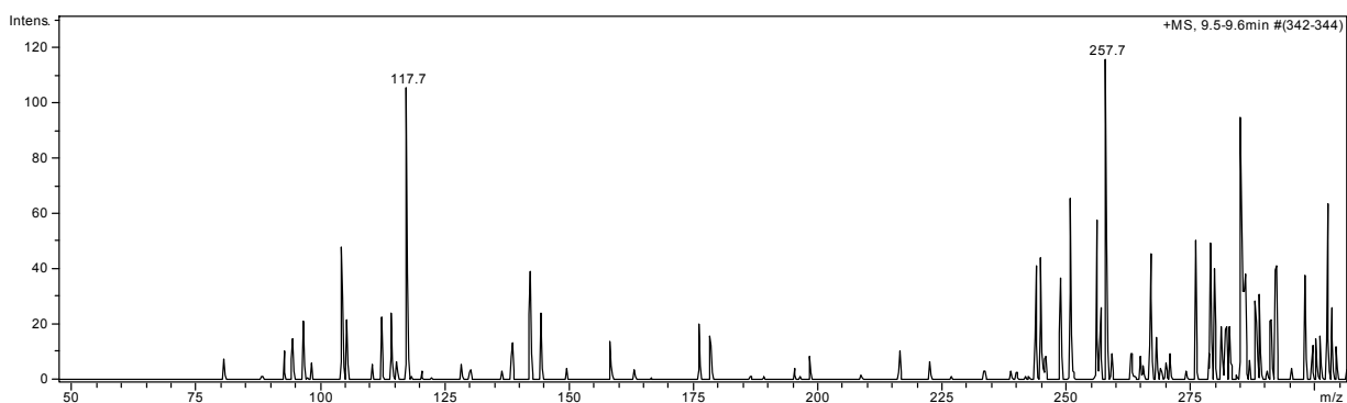
Figure 4. Valine MS-spectra
