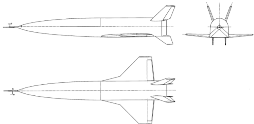
Figure 2. FTB_1 three-view
