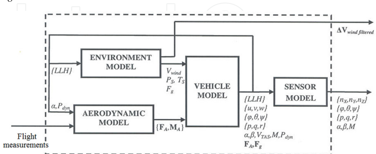
Figure 7. Filter model
