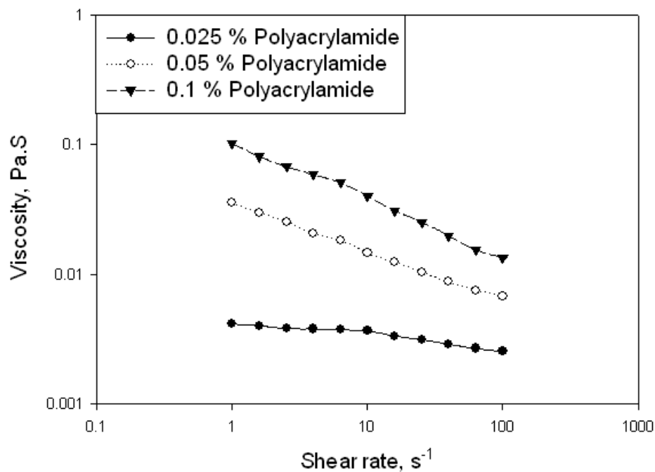
Figure 4. Viscosity versus shear rate of different concentrations of polyacrylamide solutions
