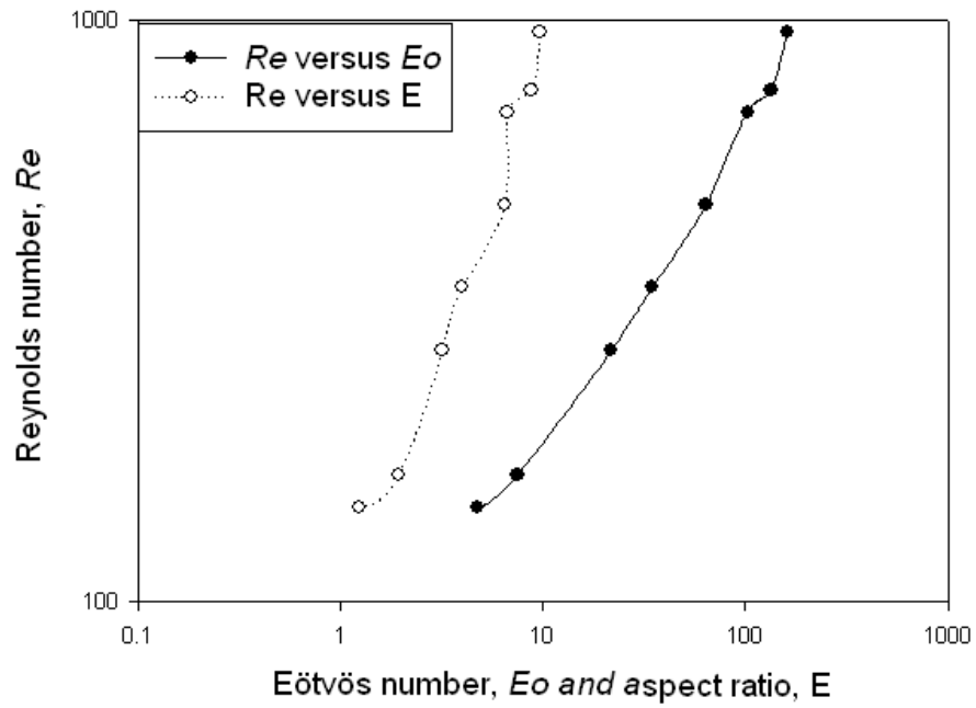
Figure 26. Re versus E_o and E for 0.05% polyacrylamide
