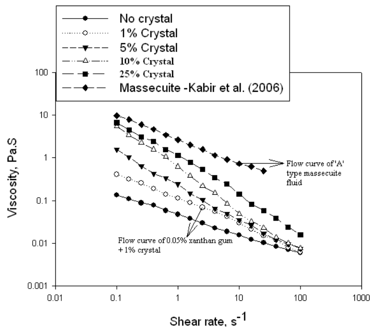
Figure 11. Viscosity versus shear rate of 0.05% xanthan gum solutions with different percentages of crystal content and massecuite of 40% crystal content at 65 °C (Hassan et al. , 2010b, Kabir et al. , 2006)
