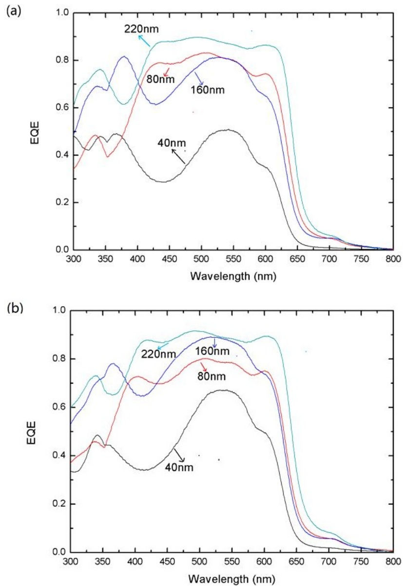
Figure 4. EQE vs. wavelength for OSC (a) and IOSC (b) with four different thicknesses of active layer: 40 nm (black), 80 nm (red), 160 nm (blue), and 220 nm (green), respectively.
