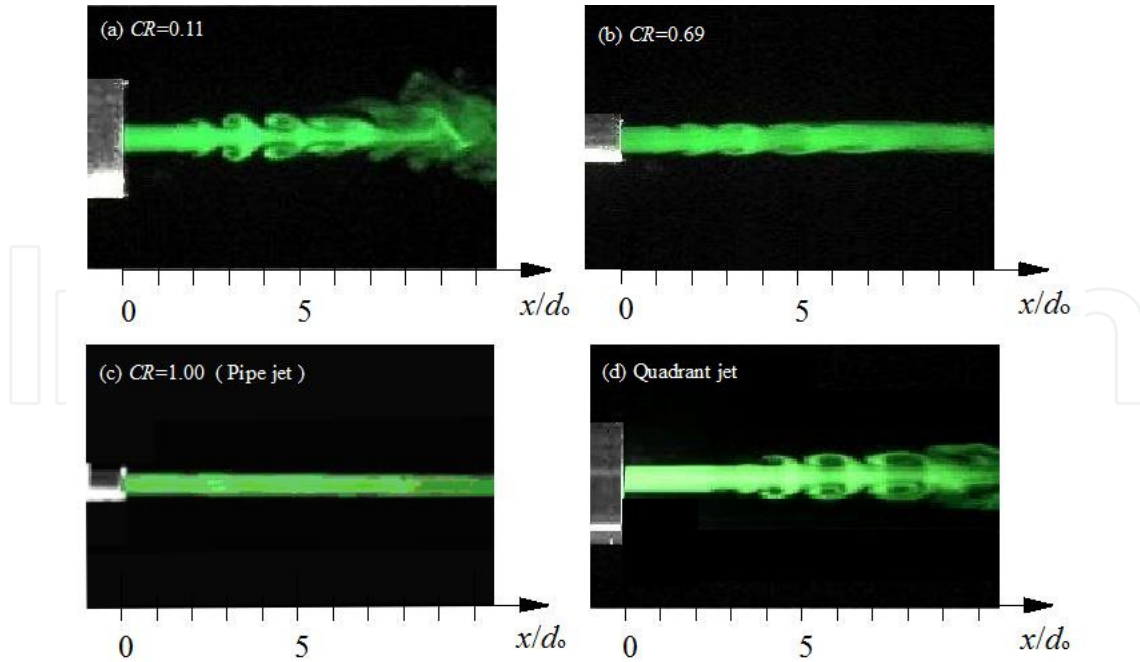
Figure 12. Flow visualization at Re=1.0 \times 10^3
