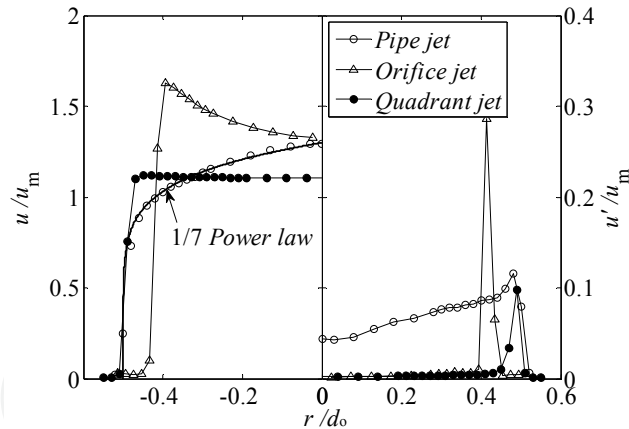
Figure 2. Mean and fluctuating velocities at the nozzle exit ( x/d_o=0.2 )
