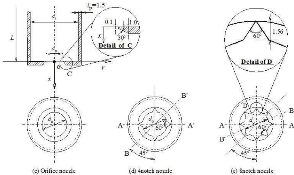
Figure 15. Nozzle configuration
