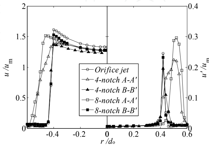
Figure 16. Mean and fluctuating velocities at the nozzle exit ( x/d_o=0.2 )
