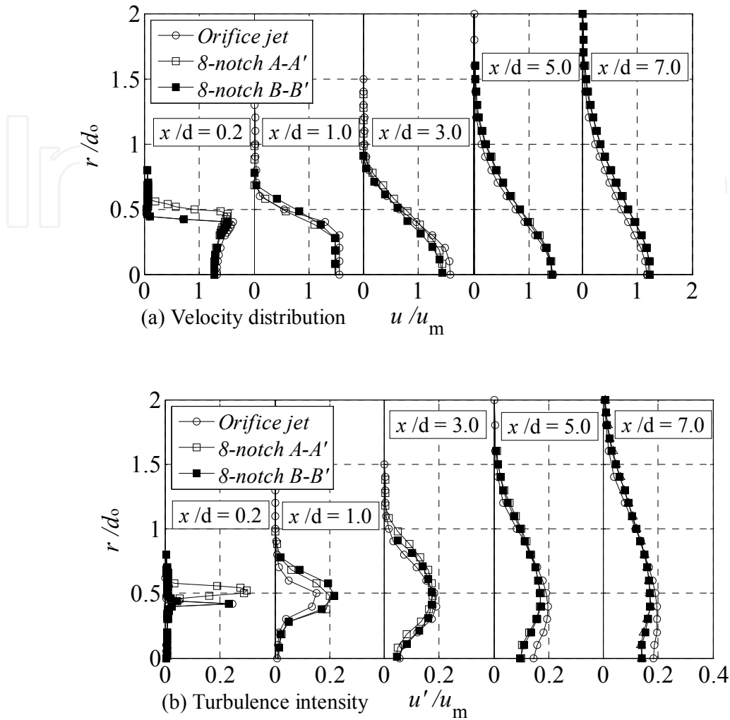
Figure 20. Centerline mean and fluctuating velocities for 8-notched orifice jet
