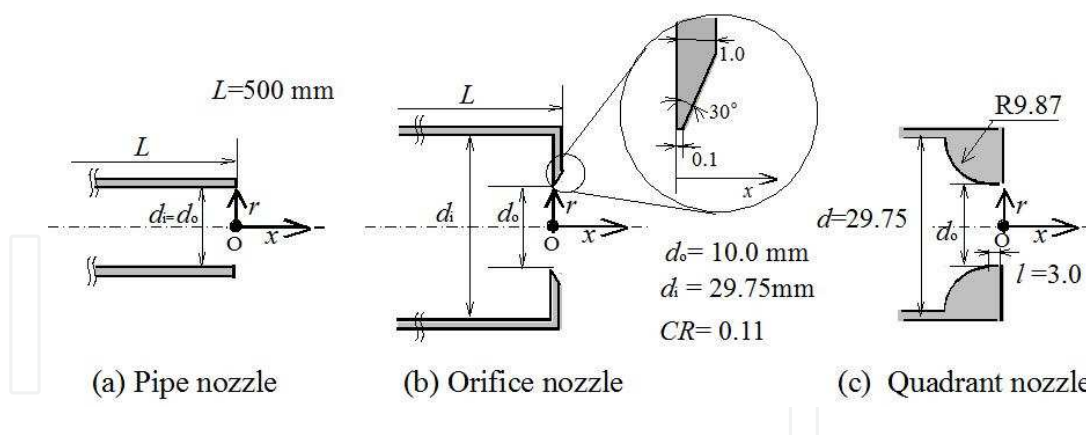
Figure 1. Nozzle configuration
