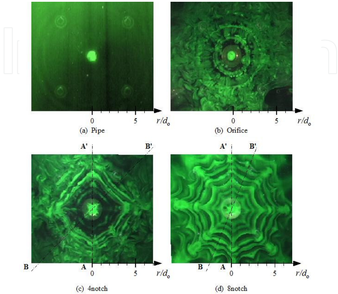
Figure 25. Flow visualization at Re=1.0 \times 10^3
