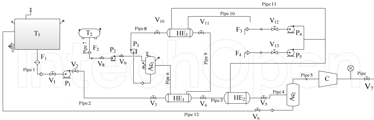
Figure 2. Regasification system
