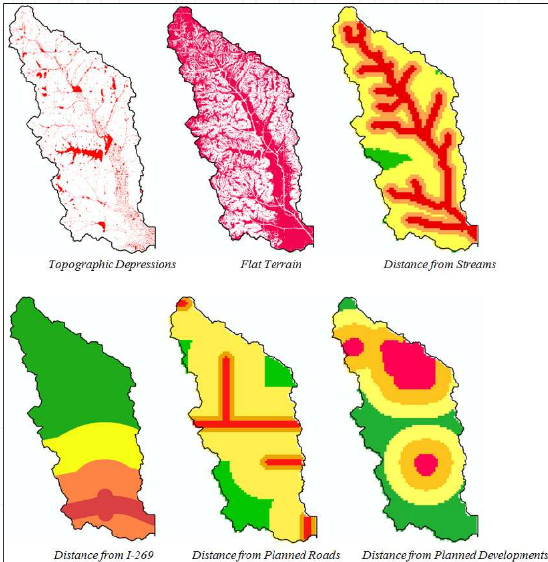
Figure 8. The layers employed to refine and rank the wetlands per watershed. For display purposes, the impact factor ranges from green (low) to red (high).
