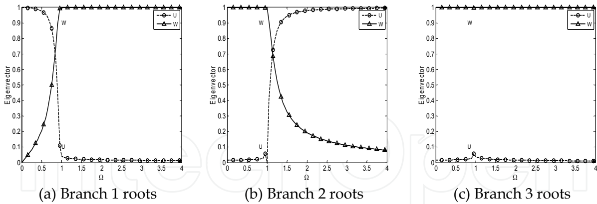
Figure 4. The normalized eigenvectors of n=0 circular harmonic (no V component)
