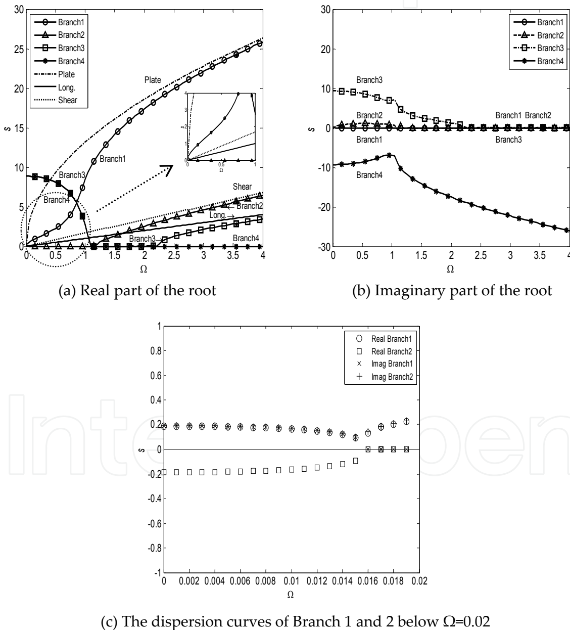
Figure 7. The dispersion relations for n=2 circular harmonic
