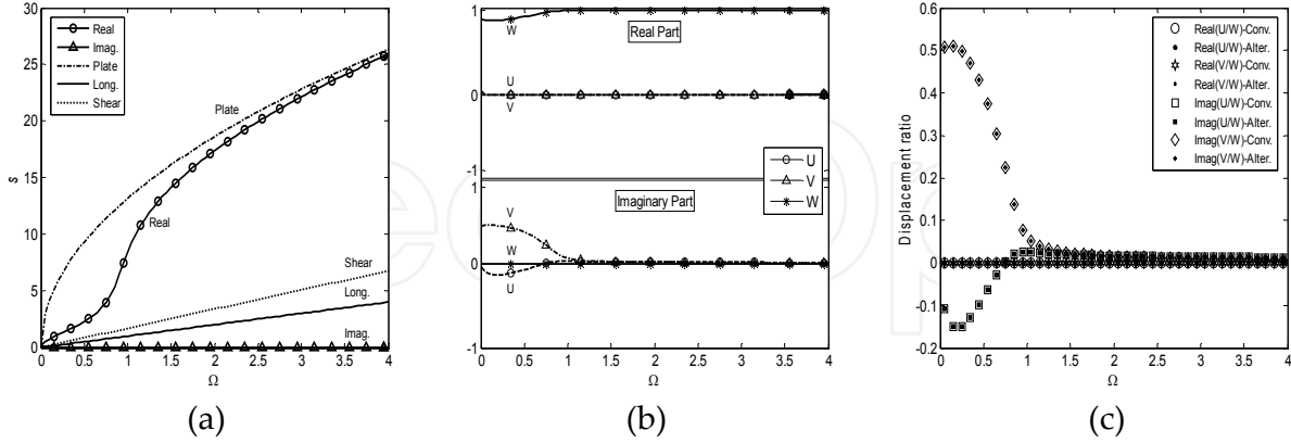
Figure 2. (a) The dispersion curve for Branch 1 roots; (b) The eigenvectors obtained from the current method expressed as [U \ V \ W]^T ; (c) Comparison between the eigenvectors (of Branch 1 roots) obtained from the conventional and the current methods ( n=2 ).
