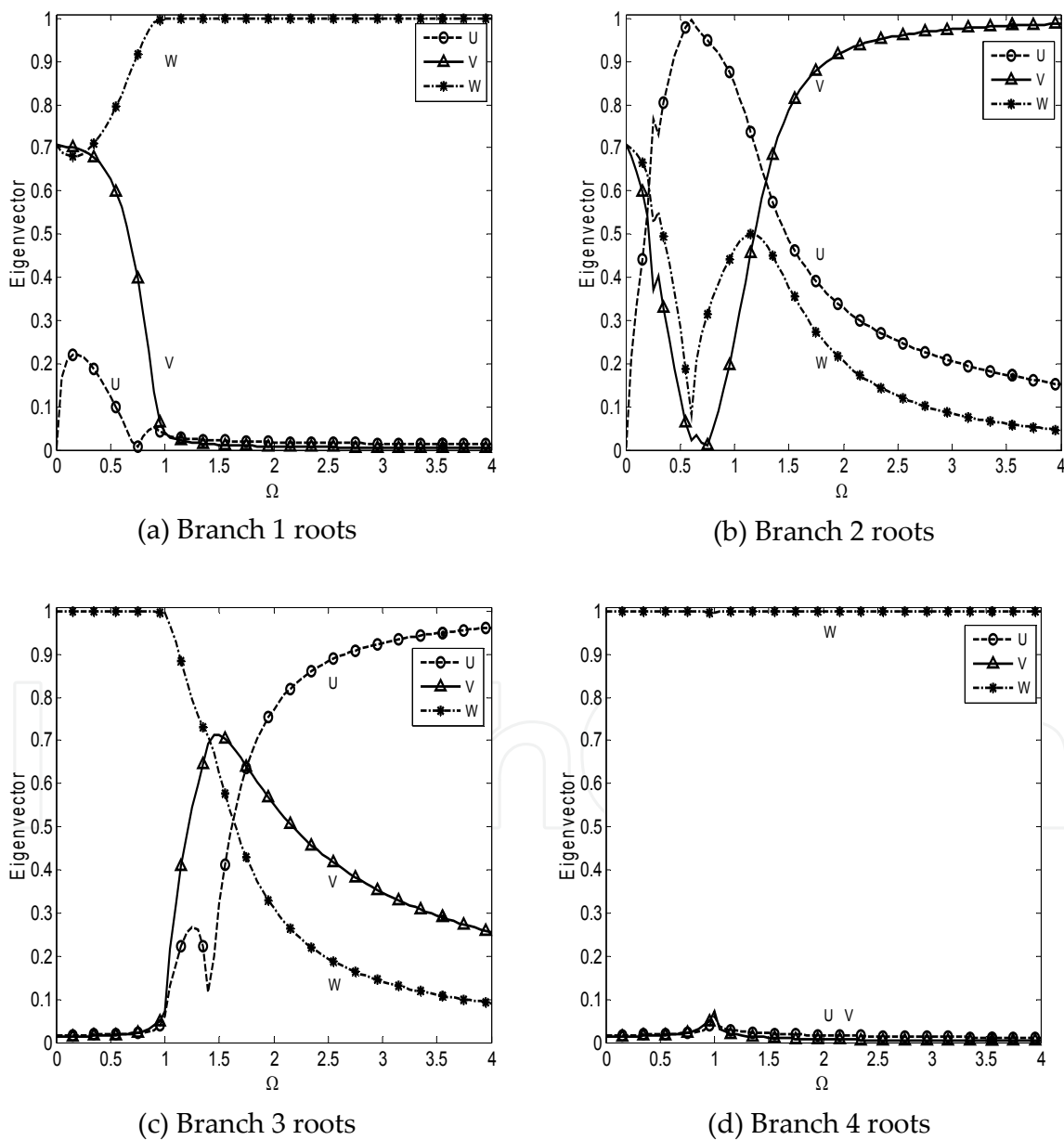
Figure 6. The normalized eigenvectors of n=1 circular harmonic.
