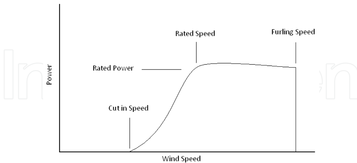
Figure 4. Turbine power versus wind speed.
