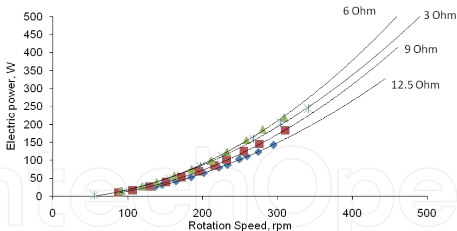
Figure 9. Power versus rotational speed for various loads
