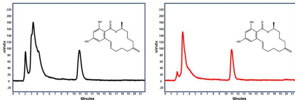
Figure 4. HPLC-FLD chromatograms of wheat sample spiked with ZON at level of 100 \mu\text{gkg}^{-1} after extract clean-up with (—) MIP-SPE (AFFINIMIP® SPE ZEARALENONE; Polyintell) and (—) immunoaffinity column (IAC).
