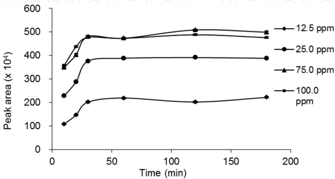
Figure 3. Effects of reaction times and concentrations on the derivatization of DNPH with 100 ng/mL MPA at room temperature.
