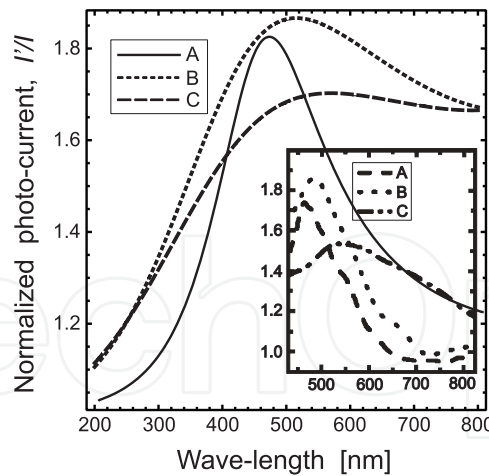
Figure 2. Dependence of the normalized photo-current I'/I(\lambda) —comparison with the experimental data [30] for A: a = 25 nm (better fitting for 19 nm), n_s = 6.6 \times 10^8 1/cm 2 , B: a = 40 nm, n_s = 1.6 \times 10^8 1/cm 2 , C: a = 50 nm, n_s = 0.8 \times 10^8 1/cm 2 ( H = 3 \mu m)
