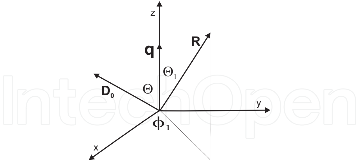
Figure 1. The reference frame is chosen in the way that the vector \mathbf{q} is oriented along the axis z , while the vector \mathbf{D}_0 lies in the plane xz
