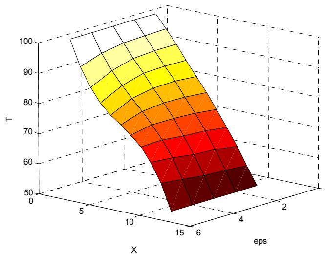
Figure 4. Graphical results of Temperature via X obtained by HPM for different values of \epsilon .
