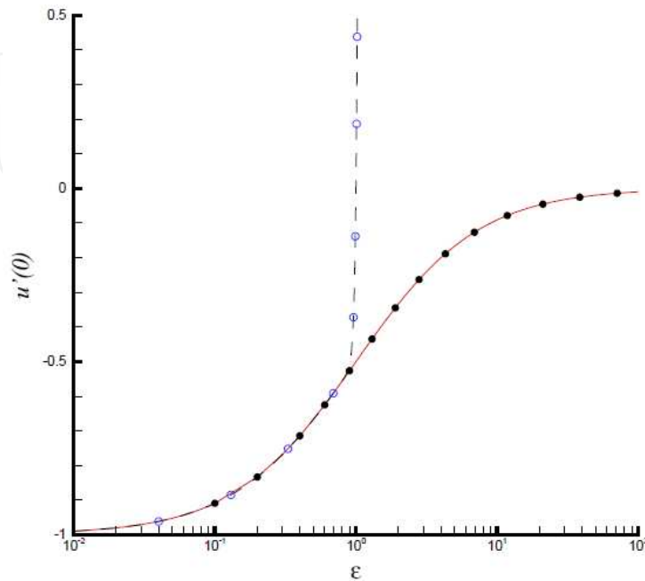
Figure 1. Comparison of the exact and approximate solutions of (1). Solid line: exact solution u'(0) = -1/(1 + \varepsilon) ; Dashed-line: 31th-order perturbation approximation; Hollow symbols: 15th-order approximation given by the HPM; Filled symbols: 15th-order approximation given by the HAM when h = -1/(1 + 2\varepsilon) .
