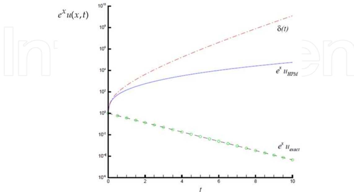
Figure 2. Approximations of (10) given by the homotopy perturbation method. Dashed-line: exact solution(12); Solid line: the 5th-order HPM approximation(17); Dash-dotted line: the relative error \delta(t) defined by(18).
