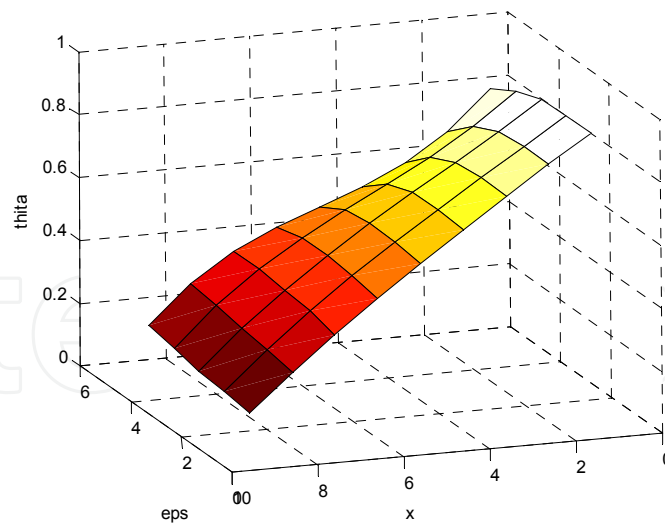
Figure 3. Graphical results \theta via X obtained by HPM for different values of \epsilon .
