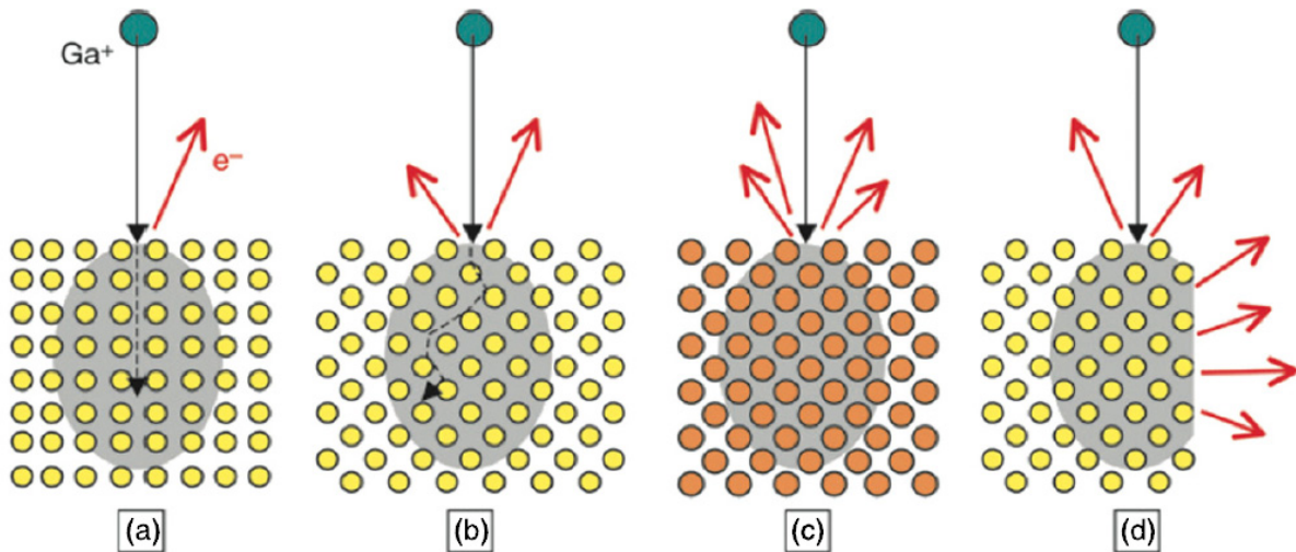
Figure 6. The crystal orientation of a sample can affect the FIB sputtering rates, shown in (a) and (b). (c) The sputtering rate is also affected by the mass of the atoms (orange atoms are more massive) and (d) by the local geometry of the sample (Lindquist et al., 2012). Original figure from Volkert et al.
