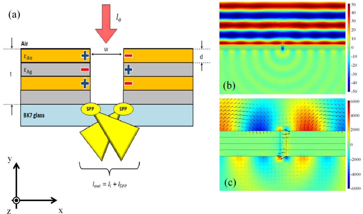
Figure 12. (a) Illustration of the adopted model. A single frequency incoming plane wave with intensity I_0 in air is linearly polarized perpendicular to a slit of subwavelength width w , milled in a multilayered metallic film with thickness t deposited on a BK7 glass substrate. Each metallic layer has a thickness d . The overall transmitted intensity I_{out} is a sum of the transmission of each layer I_i with the contribution due to the SPPs created in the air/metallic film interface I_{SPP} . (b) and (c) 2D simulations of a slit fabricated in the Au/Ag/Au/Ag film. (b) Amplitude of the magnetic H field (along the z direction). (c) Amplitude of the electric E field (in the y direction), and its vector representation in the x - y plane. Length spans: (b) x = 4 \mu\text{m} and y = 2 \mu\text{m} , and (c) x = 600 \text{ nm} and y = 400 \text{ nm} (adapted from Ferri et al., 2012)
