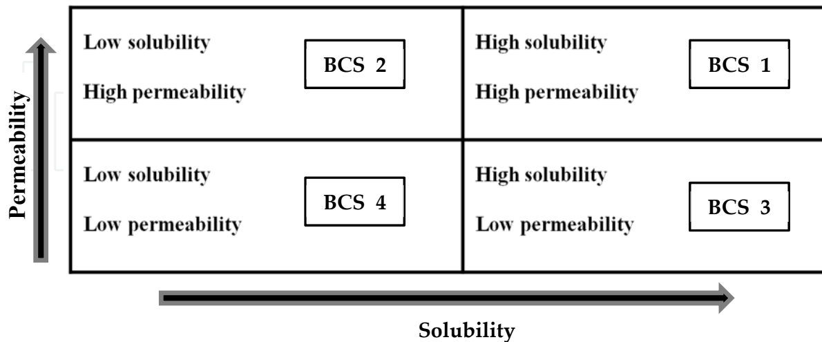
Figure 1. The Biopharmaceutical Classification System (BCS) as defined by the FDA
