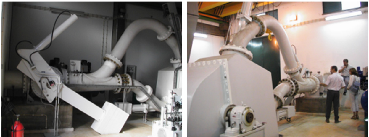
Figure 6. St. Quitéria hydropower station: inside view of Pelton turbine
