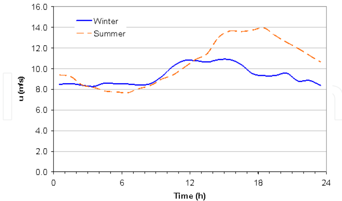
Figure 10. Wind speed average values for typical winter and summer conditions, 100 m above the ground.
