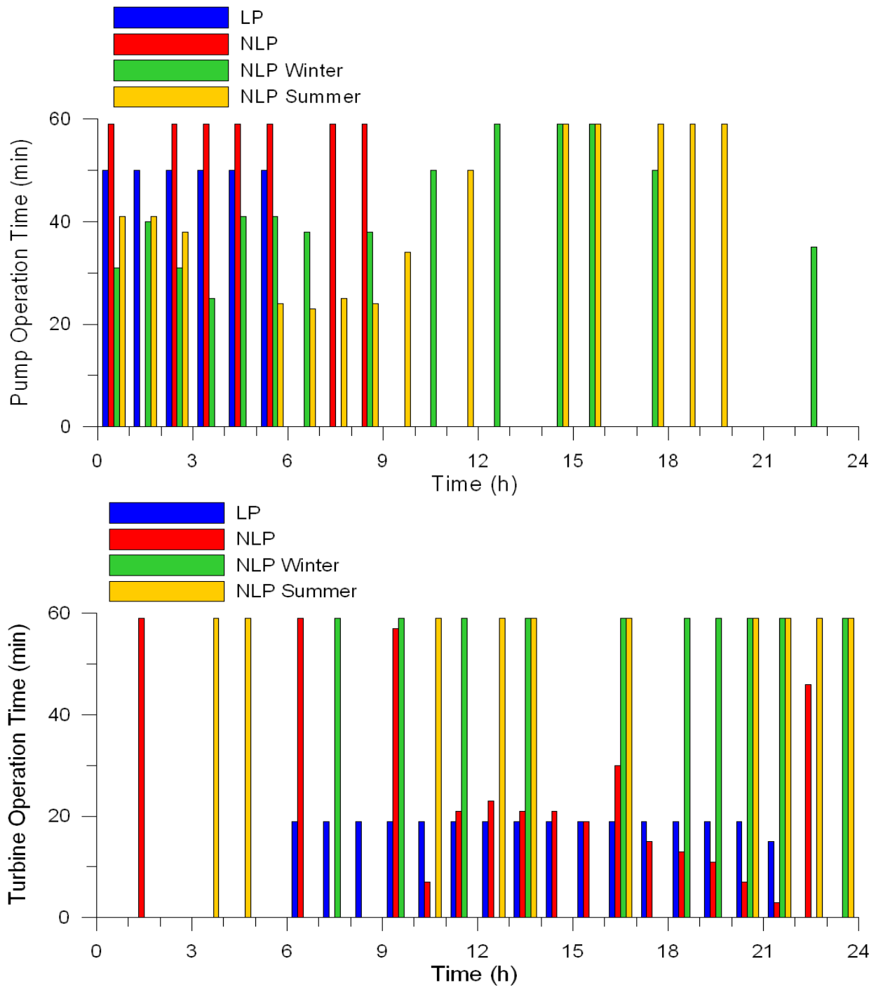
Figure 14. Pump and turbine operation time for the four modes.
