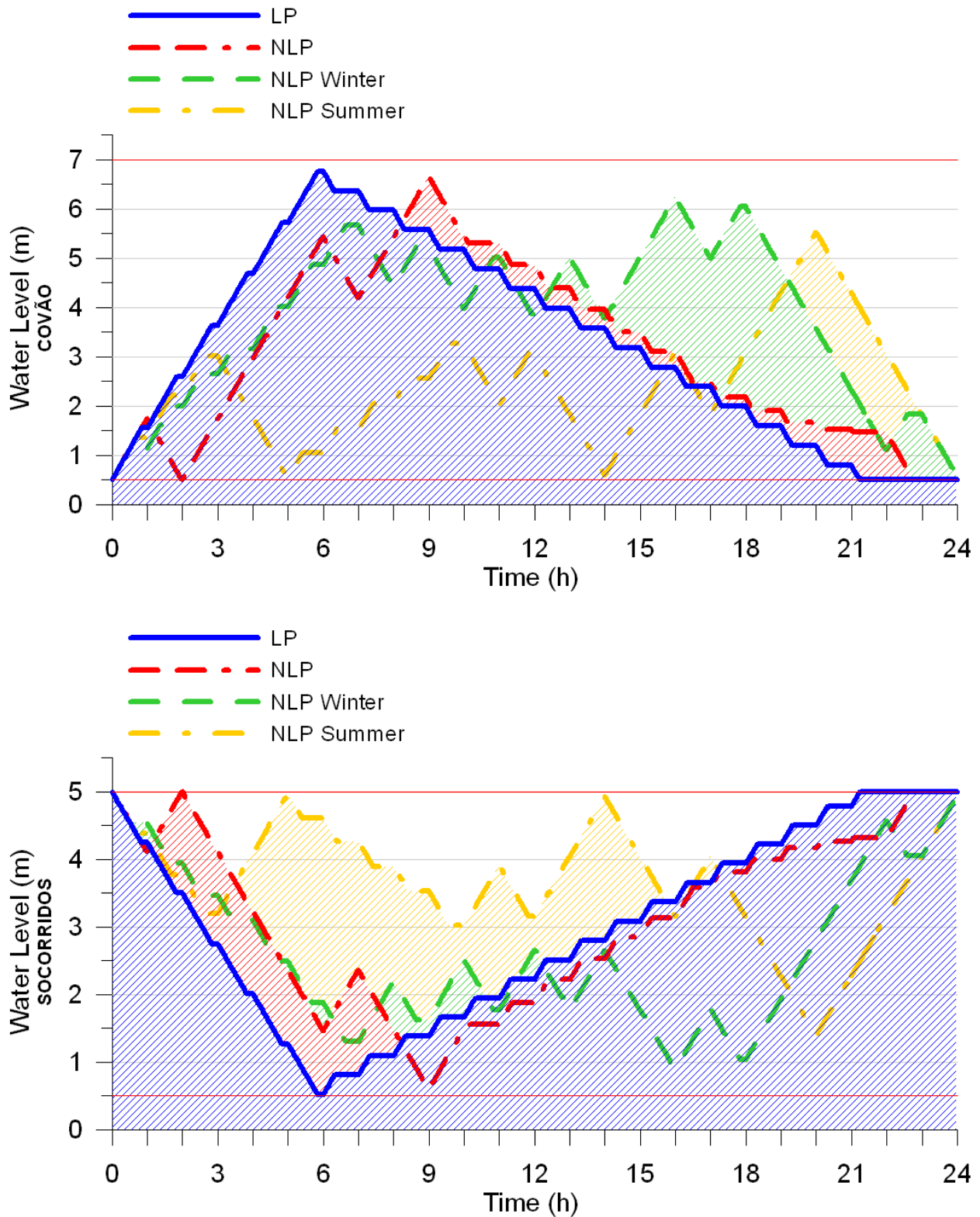
Figure 13. Water level variation in Covão and Socorridos reservoirs.
