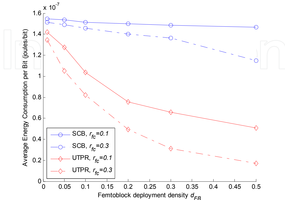
Figure 6. Average UE energy consumption per bit versus the d_{FB}
