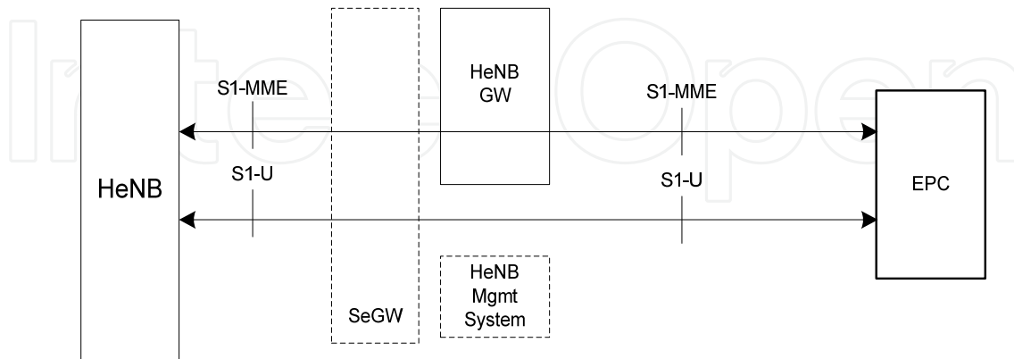
Figure 1. E-UTRAN HeNB Logical Architecture [6]
