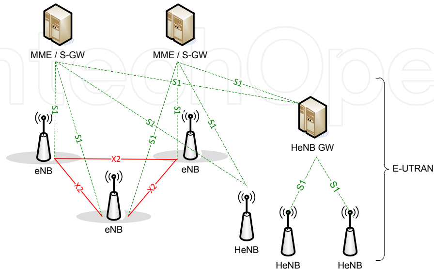
Figure 2. Support of femtocells in the LTE network architecture
