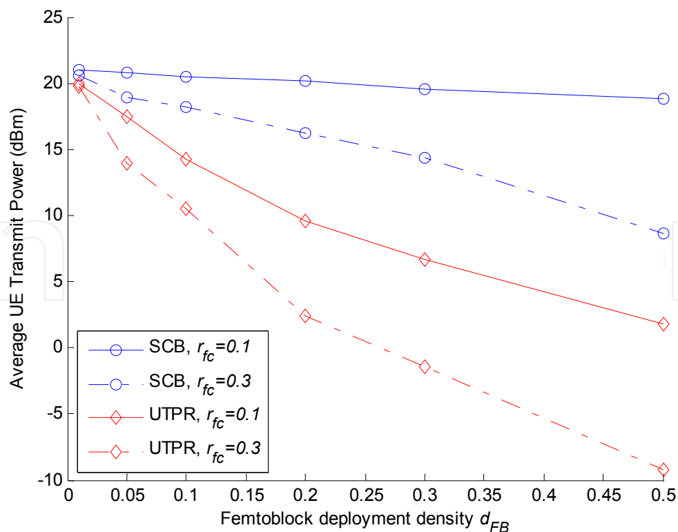
Figure 5. Average UE transmit power versus the d_{FB}
