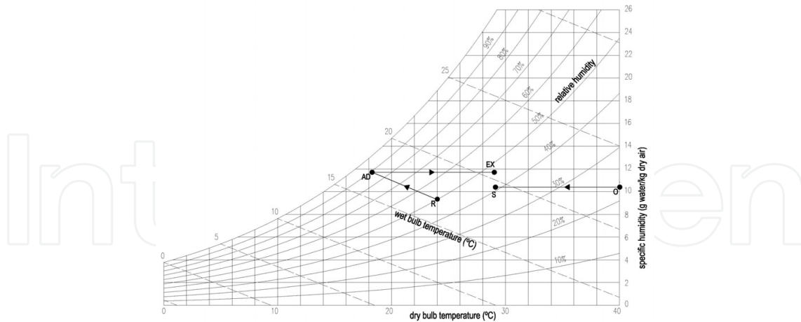
Figure 8. Psychrometric processes of indirect adiabatic cooling
