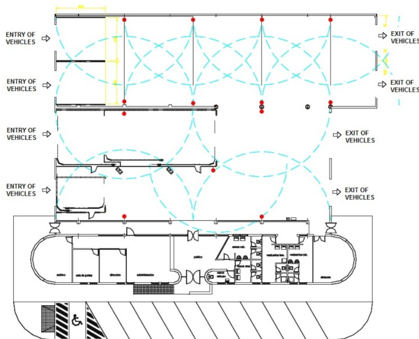
Figure 9. ITV workshop in Carmona (Seville). Plan
