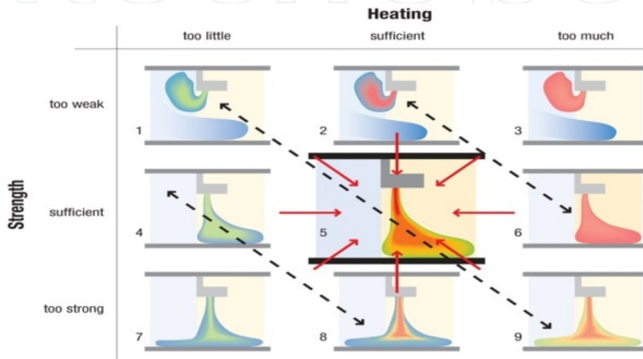
Figure 5. Air curtain strength and heating control possibilities
