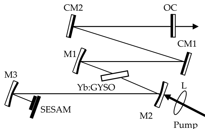
Figure 21. Cavity used to study the femtosecond laser performance of Yb:GYSO. M1, M2, M3, ROC 10\text{ cm} ; CM1, CM2, flat chirped mirrors; L, lens f=100\text{ mm} ; OC, 1\% output coupler.
