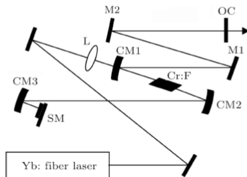
Figure 26. Schematic of the femtosecond Cr:forsterite laser. CM1–CM3: Chirped mirrors, ROC 100 mm; M1 and M2: plane chirped mirrors.
