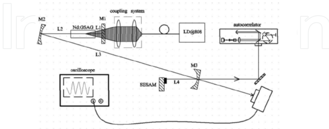
Figure 2. Schematic diagram of the experimental setup. Mirrors: M1: HT@808 nm and 1064 nm, HR@942 nm; M2: HR@942 nm, HT@1064 nm, radius of curvature (RoC)=500nm; M3: T=3%@942 nm, HT@1064 nm, RoC=100 nm.
