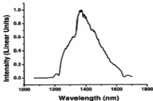
Figure 30. Emission spectrum of Cr 4+ :YAG
