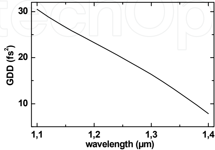
Figure 27. Group-delay dispersion from 1 mm Cr 4+ :forsterite crystal
