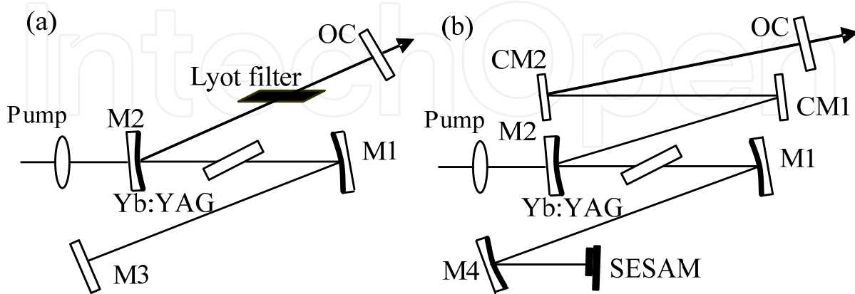
Figure 15. Cavities used to study the (a) CW and (b) mode-locked laser performance of a Yb:YAG laser.
