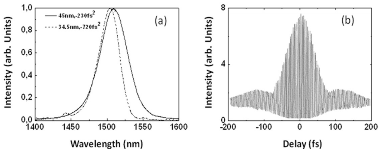
Figure 33. (a) Spectra of mode locking \text{Cr}^{4+} :YAG laser, solid curve corresponds to net GDD of -230 \text{ fs}^2 , dashed curve corresponds to -720 \text{ fs}^2 ; (b) Interferometric autocorrelation trace of mode locking pulses, the pulse duration is 65 \text{ fs} .
