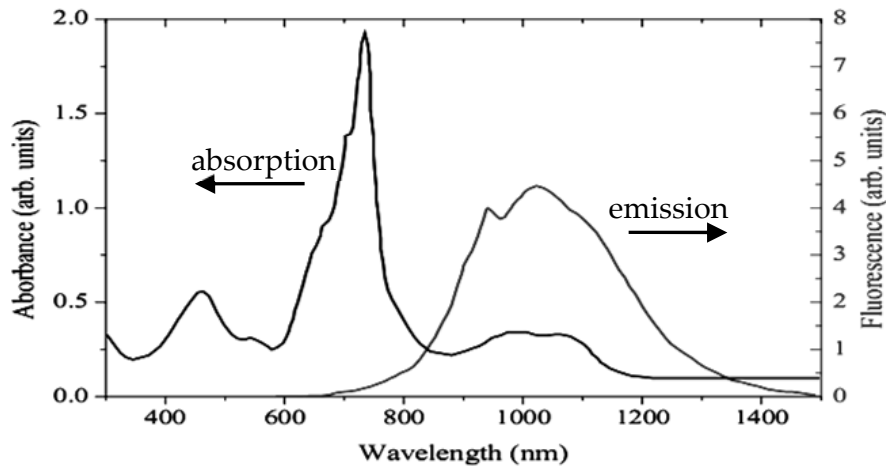
Figure 25. Absorption and emission spectrum of Cr 4+ :forsterite
