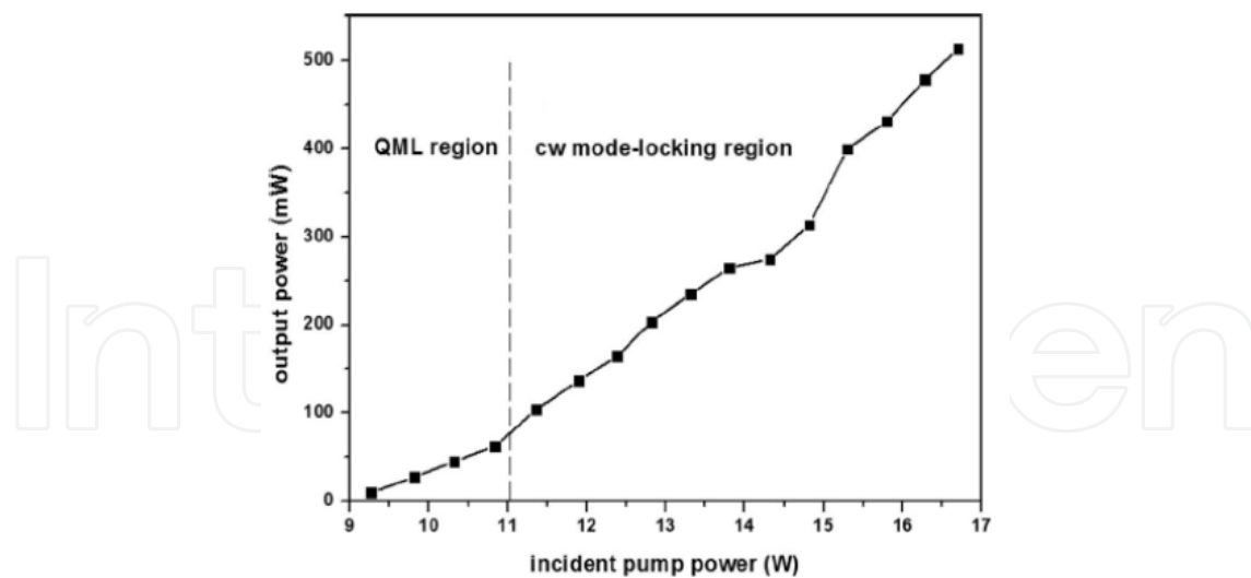
Figure 3. Dependence of the mode-locked laser output power on incident pump power.
