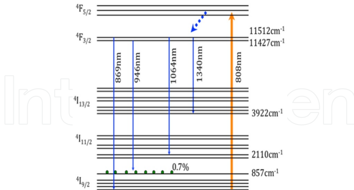
Figure 1. Energy level diagram of Nd:YAG
