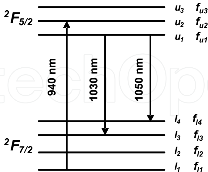
Figure 13. Energy level diagram of Yb 3+ ion in the Yb:YAG crystal.
