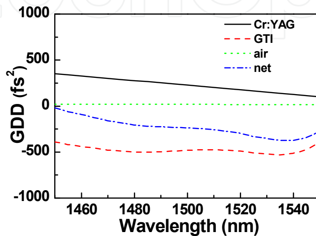
Figure 32. Intra-cavity second-order dispersion contributions.
