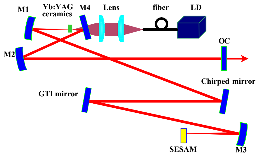
Figure 17. Schematic of the mode-locked Yb:YAG ceramic laser.
