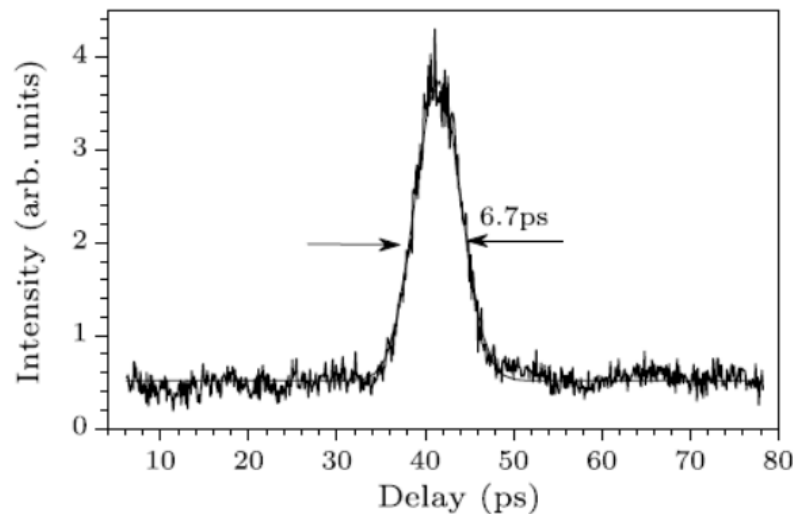
Figure 12. Autocorrelation trace of the mode-locked Nd:LuVO 4 laser.
