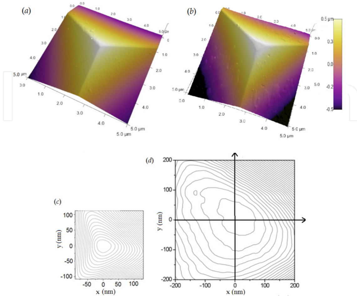
Figure 2. Three-dimensional AFM rendering image of the lightly (a) and heavily (b) used indenters, and contour plot of the surface of the lightly (c) and heavily (d) used indenter shape in the near-apex region with 2 nm contour spacing after interpolation and filtering.
