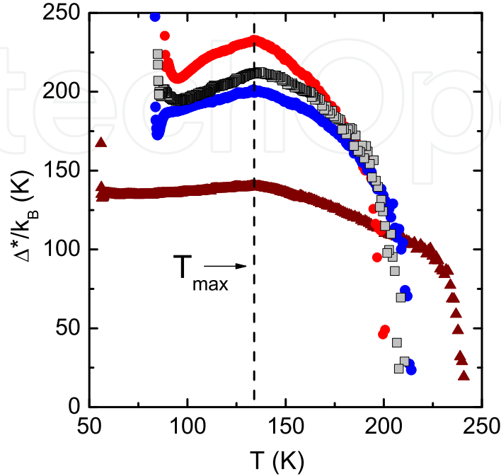
Figure 5. Dependencies of \Delta^*/k_B on T calculated by Eq. (16) for samples F1 (upper curve, circles), F3 (squares), F4 (dots) and F6 (low curve, triangles). T_{max} = T_{pair} \approx 130 K.
