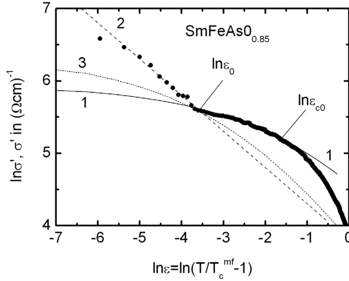
Figure 10. \ln\sigma' as a function of \ln\epsilon near T_c (dots) in comparison with the HL theory: 1-MT contribution ( d = 3.05\text{\AA} ); 2 - 3D AL contribution; 3-MT contribution ( d = 8.495\text{\AA} ).
