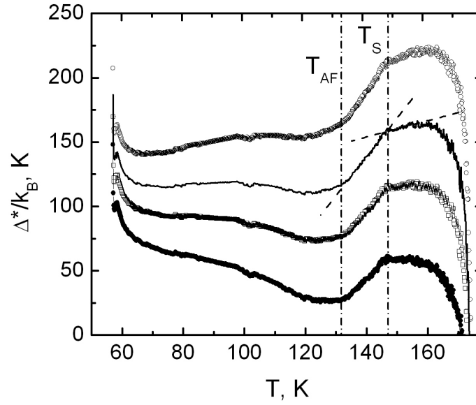
Figure 11. \Delta^*/k_B versus T dependencies for SmFeAsO_{0.85} with four different values of \Delta^*(T_c)/k_B (see the text).
