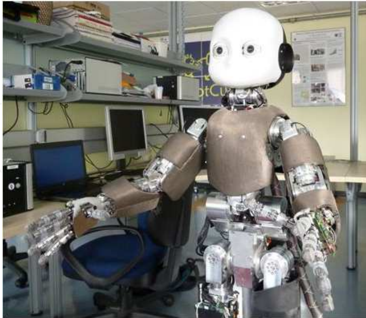
Figure 5. The iCub covered with artificial skin
