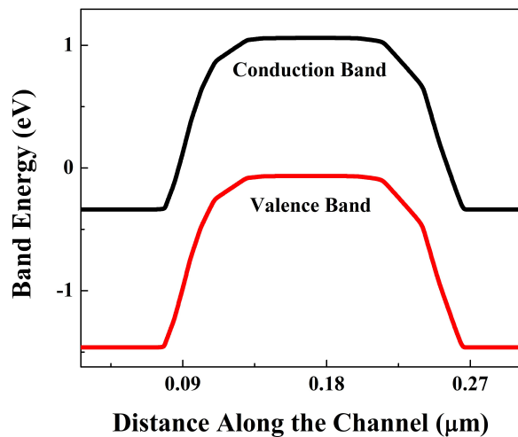
Figure 3. Energy band diagram of a tri-gate Si-FinFET.
