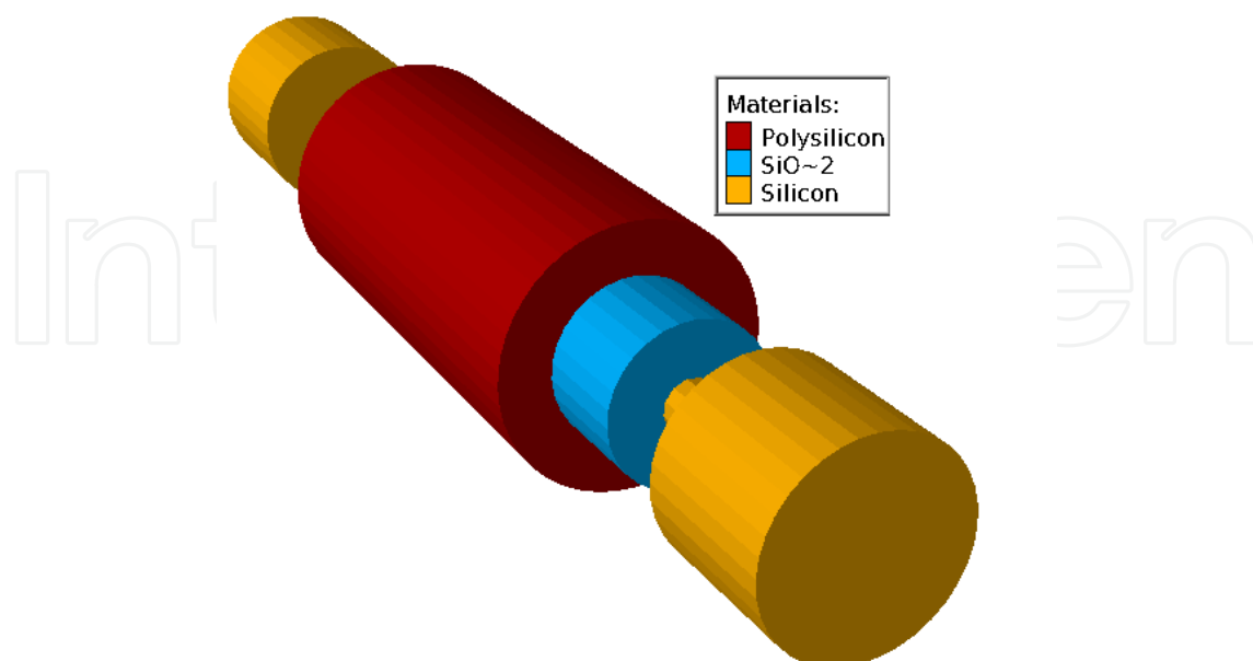
Figure 7. Simulated GAA nanowire FinFET structure.
