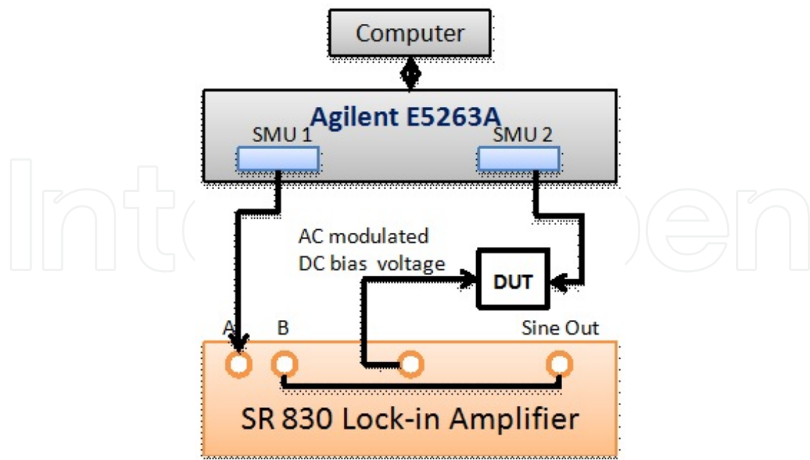
Figure 16. IETS measurement setup.
