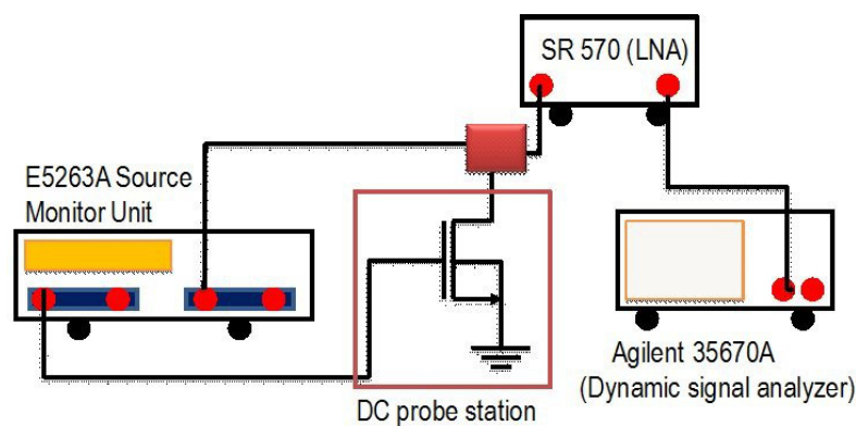
Figure 10. Low-frequency noise measurement setup.
