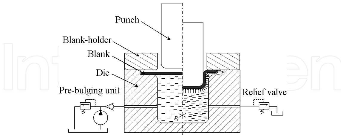
Figure 6. A simplified schematic of tool set-up for hydrodynamic deep drawing [16]
