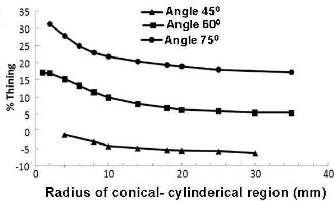
Figure 46. % thinning versus radius of conical-cylindrical region
