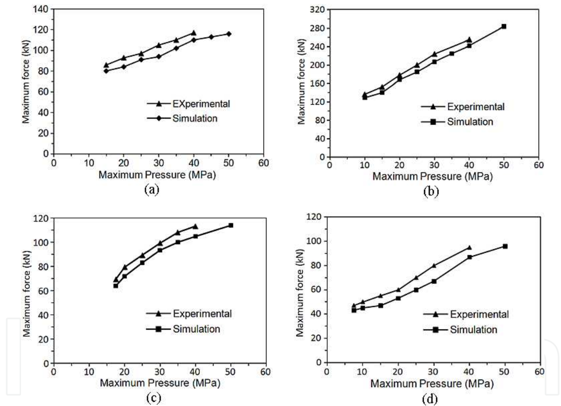
Figure 35. Maximum punch force versus maximum pressure corresponding to (a) Part A, (b) Part B, (c) Part C, (d) Part D
