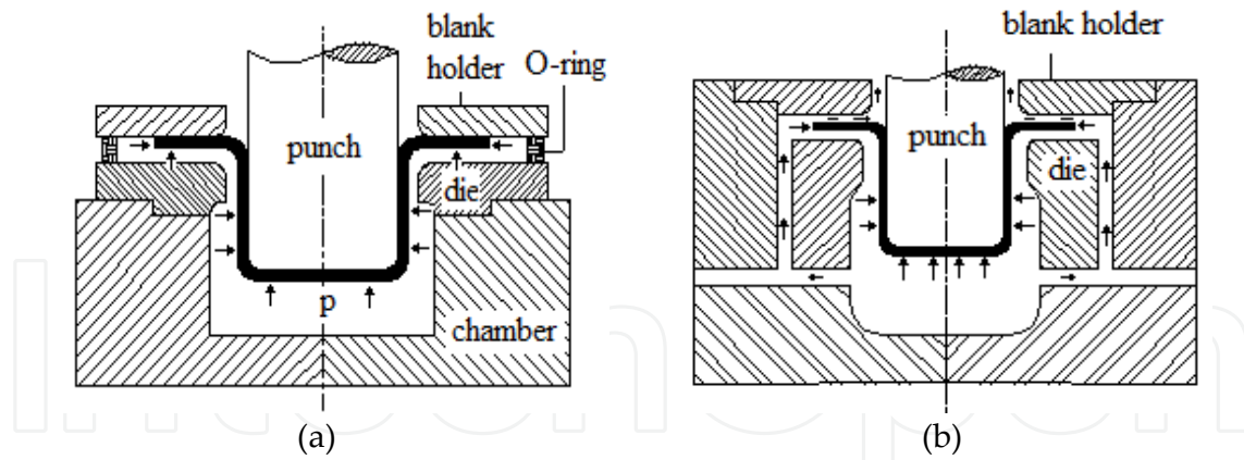
Figure 4. Tool set-up for: (a) hydromechanical, (b) hydro-rim, deep drawing process [9]
