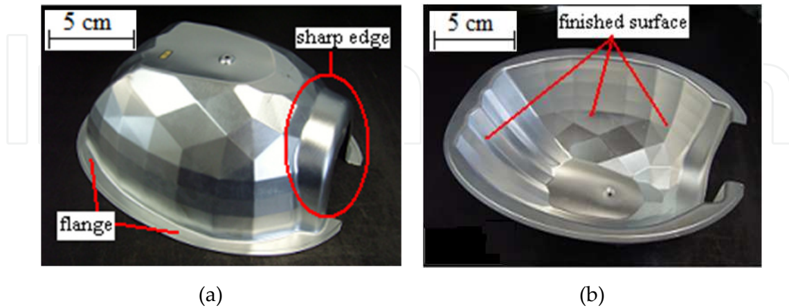
Figure 7. Case study 1; The part of lightning industry (after trimming and coating): (a) internal view, (b) external view
