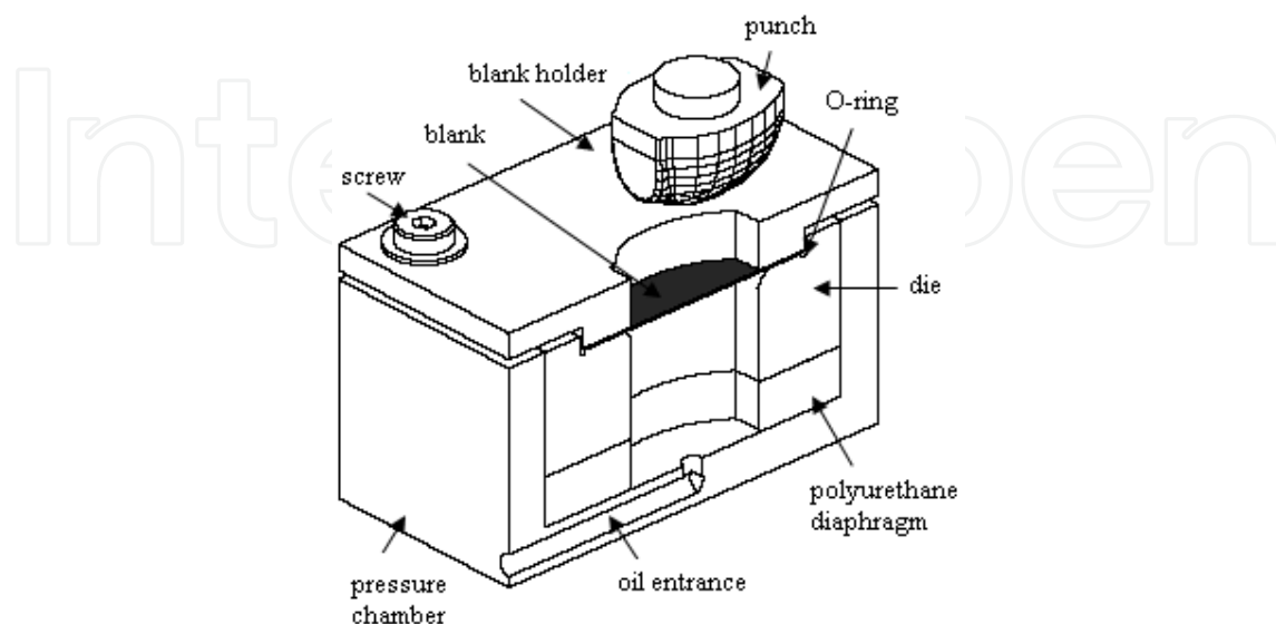
Figure 19. Schematic illustration of the proposed set-up for a complex part
