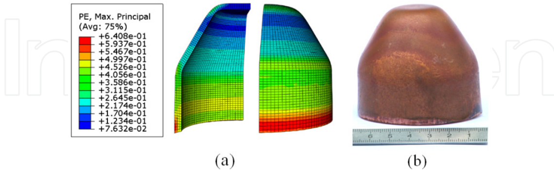
Figure 27. Deformed part A corresponds to pressure path 25 MPa, (a) simulation, (b) experiment
