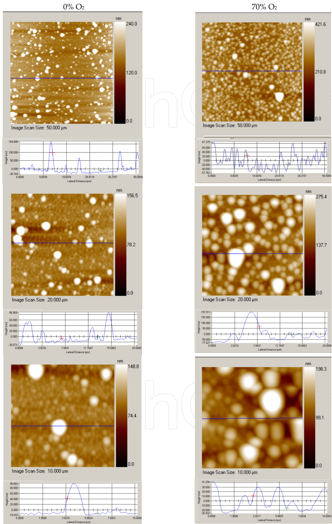
Figure 4. Surface topographical images of the sample deposited in pure HMDSO (left) and in HMDSO/O 2 (right) plasmas acquired at different magnifications.
