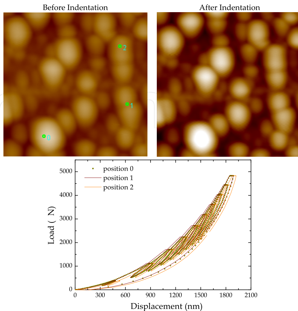
Figure 8. 10 \times 10 \mu\text{m}^2 atomic force microscopy images of the film deposited in plasmas of HMDSO/ \text{O}_2 mixtures: (left) prior and (right) after indentation. The points in the left image correspond to the location where the indentations were conducted using 5000 \mu\text{N} of maximum load in a multiple load function. The lower graph presents the loading-displacement functions generated in each corresponding point.
