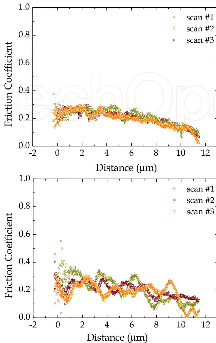
Figure 17. Friction coefficient as a function of the position for the films prepared in pure HMDSO (left) and HMDSO/O 2 (right) plasma. The scans were acquired at 300 \mu\text{N} of normal load and at a velocity of 1.0 \mu\text{m/s} .
