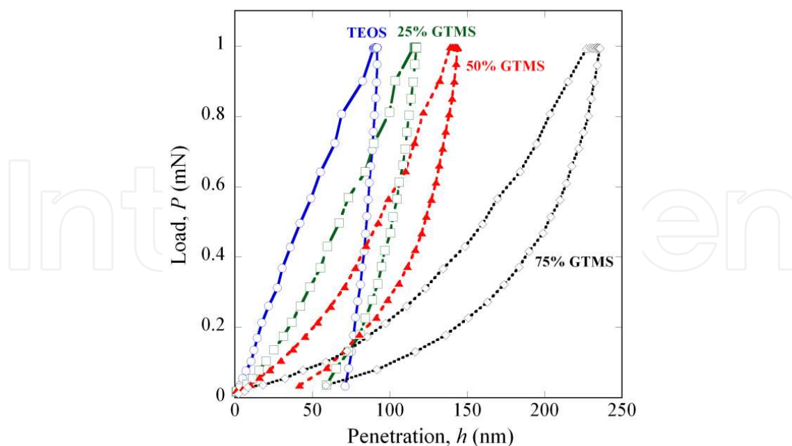
Figure 8. Indentation load-displacement curves for TEOS and GTMS on Cu substrates. P = 1 mN with 10 s dwell at maximum force [Redrawn from ref (Latella et al., 2008a)].
