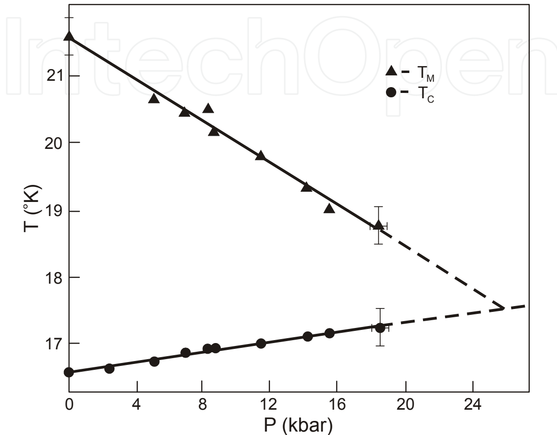
Figure 1. Schematic representation of the temperature dependence with pressure showing the critical temperature and martensitic temperature for V_3Si .
