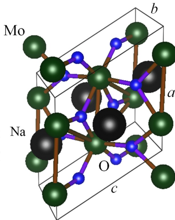
Figure 11. Crystalline structure of the A_x\text{MoO}_{2-\delta} with A = \text{Na} or \text{K} .
