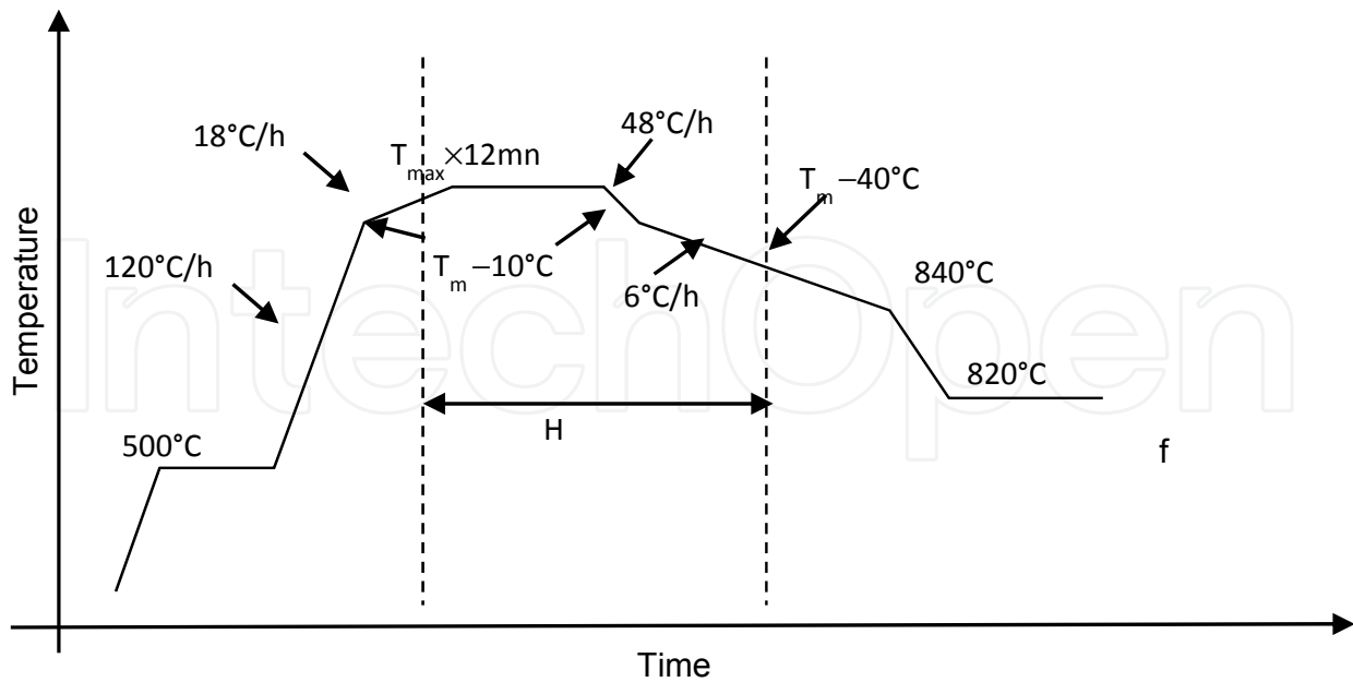
Figure 6. Generalized temperature profile for MMP \text{Bi}_2\text{Sr}_2\text{CaCu}_2\text{O}_{8+x} tapes in magnetic field up to 15T [26]. T_{\text{max}} is the maximal annealing temperature. The magnetic field is applied at T_{\text{max}} and shut down at T_{\text{max}} - 40^\circ\text{C} . The atmosphere is flowing \text{O}_2 .
