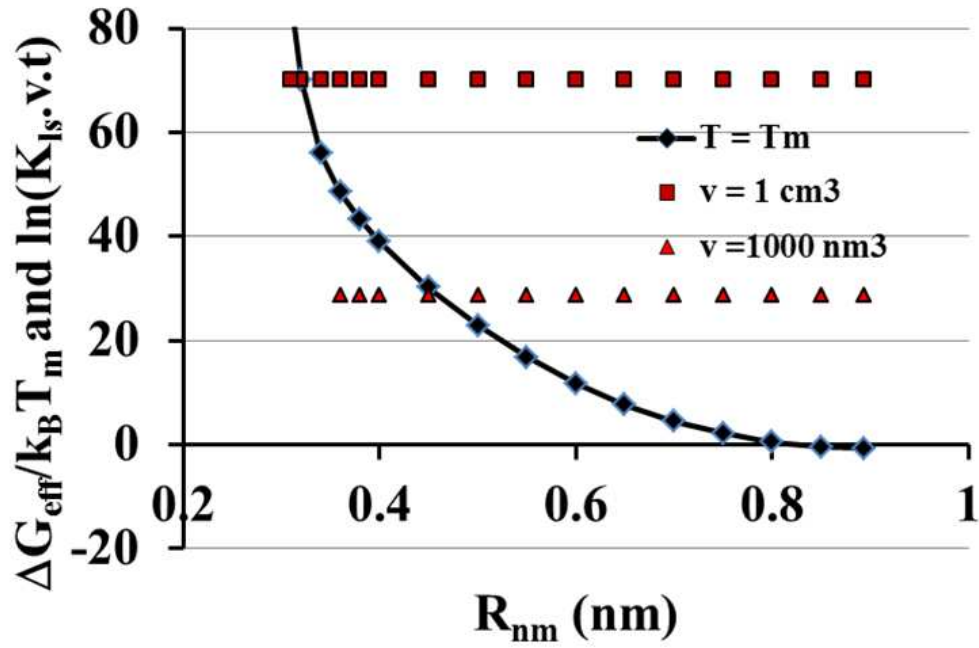
Figure 12. The difference (\Delta G_{21s}^*/k_B T_m - \Delta G_{nm}/k_B T_m = \Delta G_{\text{eff}}/k_B T_m) , the \ln(K_{1s} \cdot v \cdot t) = 70.1 with v = 10^{-6} \text{ m}^3 , K_{1s} = 76.4 , t_{sn} = 1800 \text{ s} , and \ln(K_{1s} \cdot v \cdot t) = 28.6 with K_{1s} = 76.4 , v = 10^{-24} \text{ m}^3 and t_{sn} = 1800 \text{ s} are represented as a function of the surviving nucleus radius R_{nm} . All nuclei with 0.45 < R_{nm} < 0.894 \text{ nm} can grow at T = T_m in a sample volume of 10^{-24} \text{ m}^3 using our model of identical atoms.
