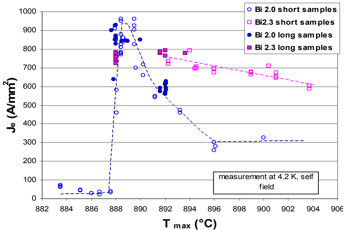
Figure 7. Critical current density in \text{Bi}_2\text{Sr}_2\text{CaCu}_2\text{O}_{8+x} Ag-sheathed tapes as a function of maximal temperatures [34] for two different compositions. Pre-reacted \text{Bi}_2\text{Sr}_2\text{CaCu}_2\text{O}_{8+x} powders are used.
