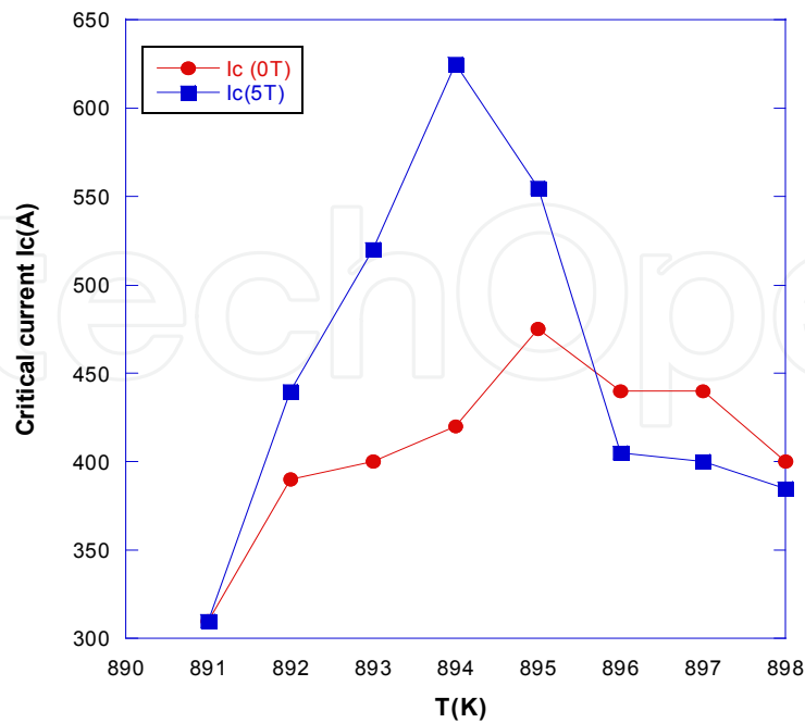
Figure 9. Critical current in Ag sheathed tapes of Bi_2Sr_2CaCu_2O_{8+x} as a function of maximal annealing temperature measured at 4.2K with field and without field [35].
